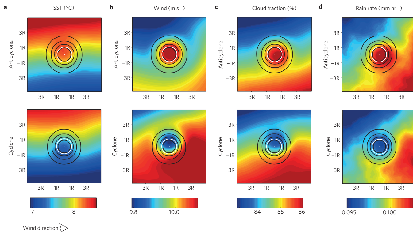
Figure 2 | Mean eddy and pattern of its atmospheric imprint. a , SST ( \pm 0.04^\circ\text{C} ). b , Wind speed ( \pm 0.01\text{ m s}^{-1} ). c , Cloud fraction ( \pm 0.1\% ). d , Rain rate ( \pm 10^{-3}\text{ mm h}^{-1} ). Shown are mean composite maps of the >600,000 individual eddy realizations south of 30^\circ\text{S} , divided into anticyclones and cyclones. White circles mark the eddy core as detected with the Okubo–Weiss parameter and black lines denote sea level anomaly contours associated with the eddy. Before averaging, the eddies were scaled according to their individual eddy amplitude and radius ( R ), interpolated and rotated so that the large-scale wind is from left to right.
