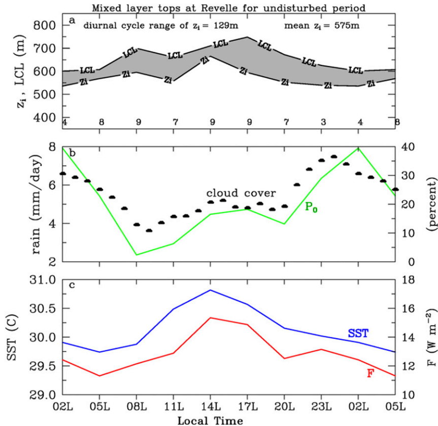
FIG. 13. (a) Diurnal cycle of mixed-layer depth z_i (m) and LCL based on mixed-layer-mean conditions, (b) mean radar-determined rainfall rate P_0 (green) in TOGA radar range and ceilometer-estimated cloud cover (cloud symbols), and (c) mean SST (blue) and surface buoyancy flux F (red) for November undisturbed period at Reville . Gray shading in (a) indicates difference between LCL and z_i . Diurnal cycle range and mean value of z_i , along with numbers of soundings at each time (on bottom axis), are shown in (a).
