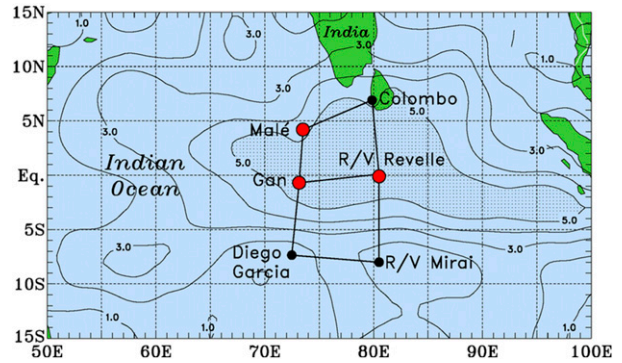
FIG. 1. DYNAMO enhanced sounding network for the period October–December 2011. Analyses of mixed layers have been carried out on soundings from Malé ( 4\text{ day}^{-1} ), Gan Island ( 8\text{ day}^{-1} ), and Revelle ( 8\text{ day}^{-1} ) (red dots), which constituted part of the northern sounding array. That array experienced a stronger MJO signal than the southern array as indicated by amplitude of 20-day low-pass-filtered 450-hPa vertical motion (contours; \text{hPa h}^{-1} , values >5\text{ hPa h}^{-1} are stippled). Colombo data were not used because of significant island influences.
