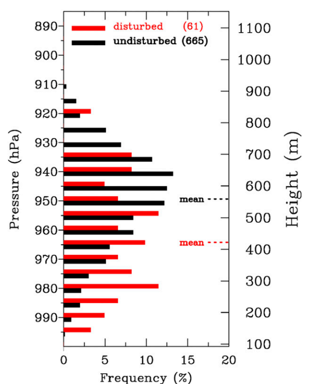
FIG. 5. Histograms of mixed-layer depth at Gan Island for undisturbed (black) and disturbed (red) periods for the full duration of DYNAMO (1 Oct 2011–8 Feb 2012) using 5-hPa bins. See text for definitions. Horizontal dashed lines indicate mean values. Numbers of mixed-layer cases are in parentheses.
