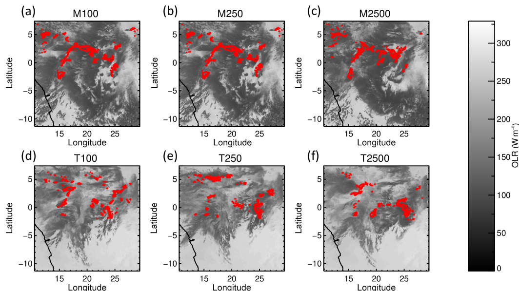
Figure 1. Congo case: instantaneous outgoing longwave radiation ( \text{W m}^{-2} , greyscale) and 5 \text{ mm h}^{-1} surface precipitation rate (red contour) at 07:00 UTC on 7 August 2007 in the Congo basin configuration. (a–c) CONGO-MORR simulations and (d–f) CONGO-THOM simulations. Prescribed CDNC values of 100, 250 and 2500 \text{ cm}^{-3} are shown in panels (a, d), (b, e) and (c, f), respectively.
