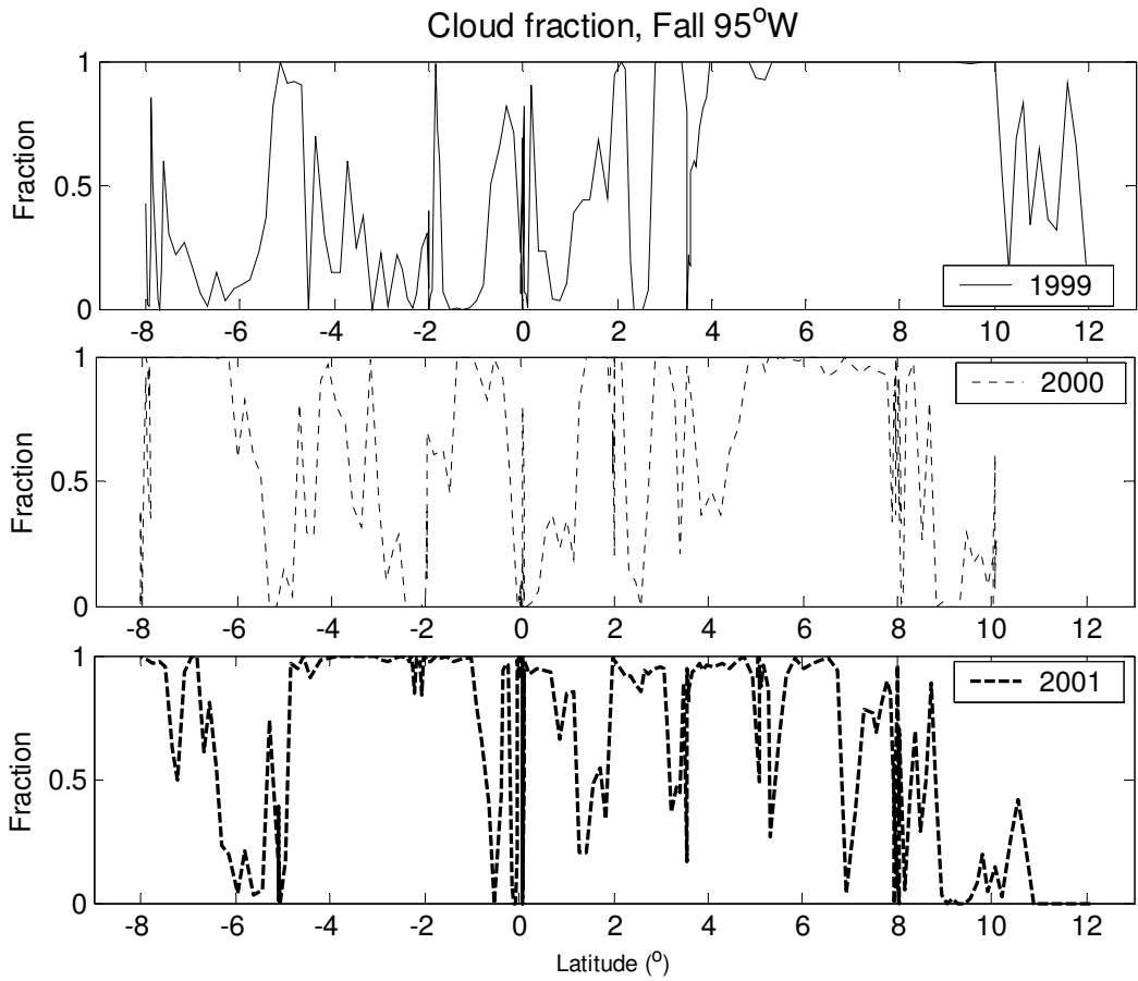
Figure 9 – Ceilometer measured cloud fraction for fall seasons.
