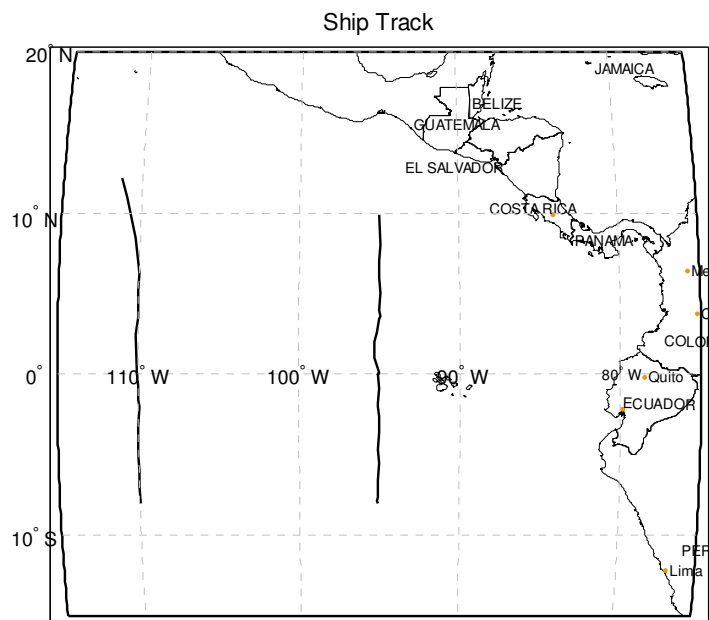
Figure 2—Track of research vessel during cruises from 1999-2001
