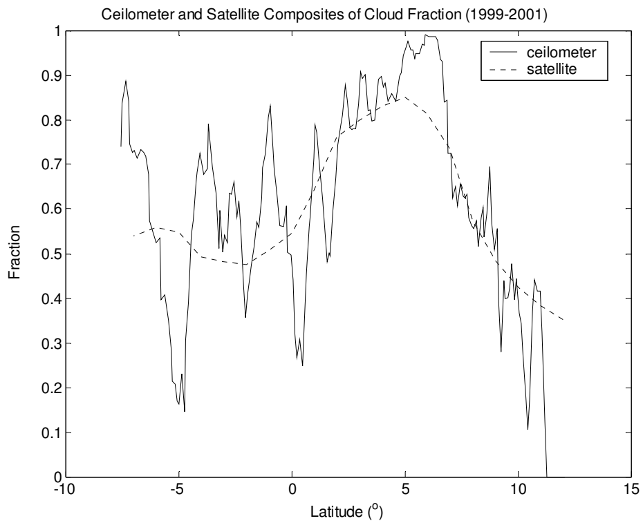
Figure 13 – Ceilometer (solid) and satellite (dash) composite comparison of fractional cloudiness.
