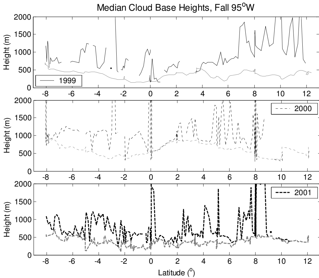
Figure 10 – Ceilometer measured cloud base height (black) and LCL (gray) for fall seasons.
