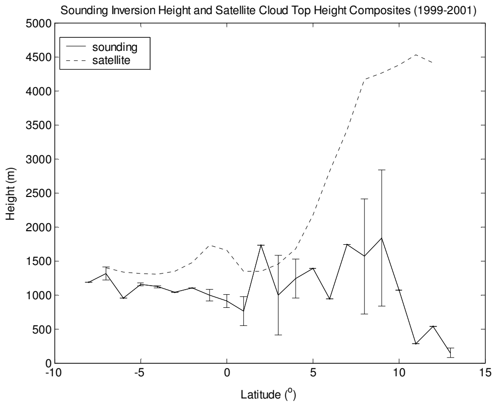
Figure 14—Inversion heights from soundings (1999-2001) and satellite cloud top height composite. Error bars are the standard deviation of the average inversion height in each latitude bin.
