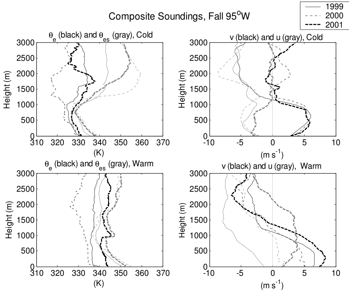
Figure 8 – Composite soundings for the fall seasons 1999-2001 on the 95°W transect. The top 2 panels are from the cold (4°S-0°N) side of the SST gradient and the bottom 2 panels are from the warm (2°-6°N) side of the gradient.
