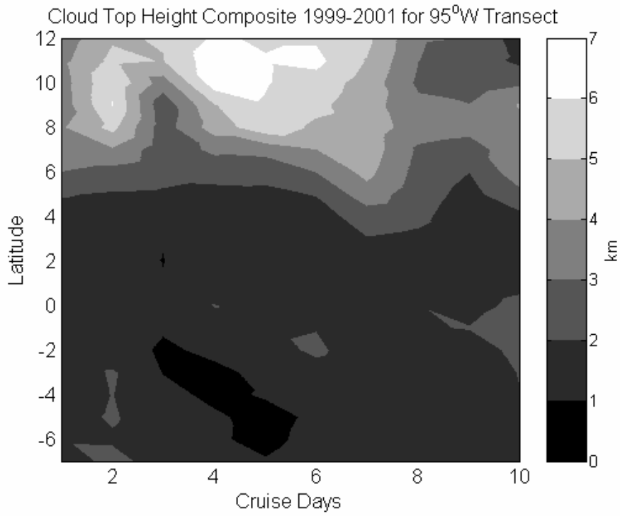
Figure 12—Satellite derived cloud top height composite for 1999-2001.
