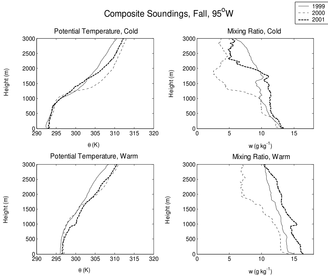
Figure 7 -- Composite soundings for the fall seasons 1999-2001. The top 2 panels are from the cold (4°S-0°N) side of the SST gradient and the bottom 2 panels are from the warm (2°-6°N) side of the gradient.
