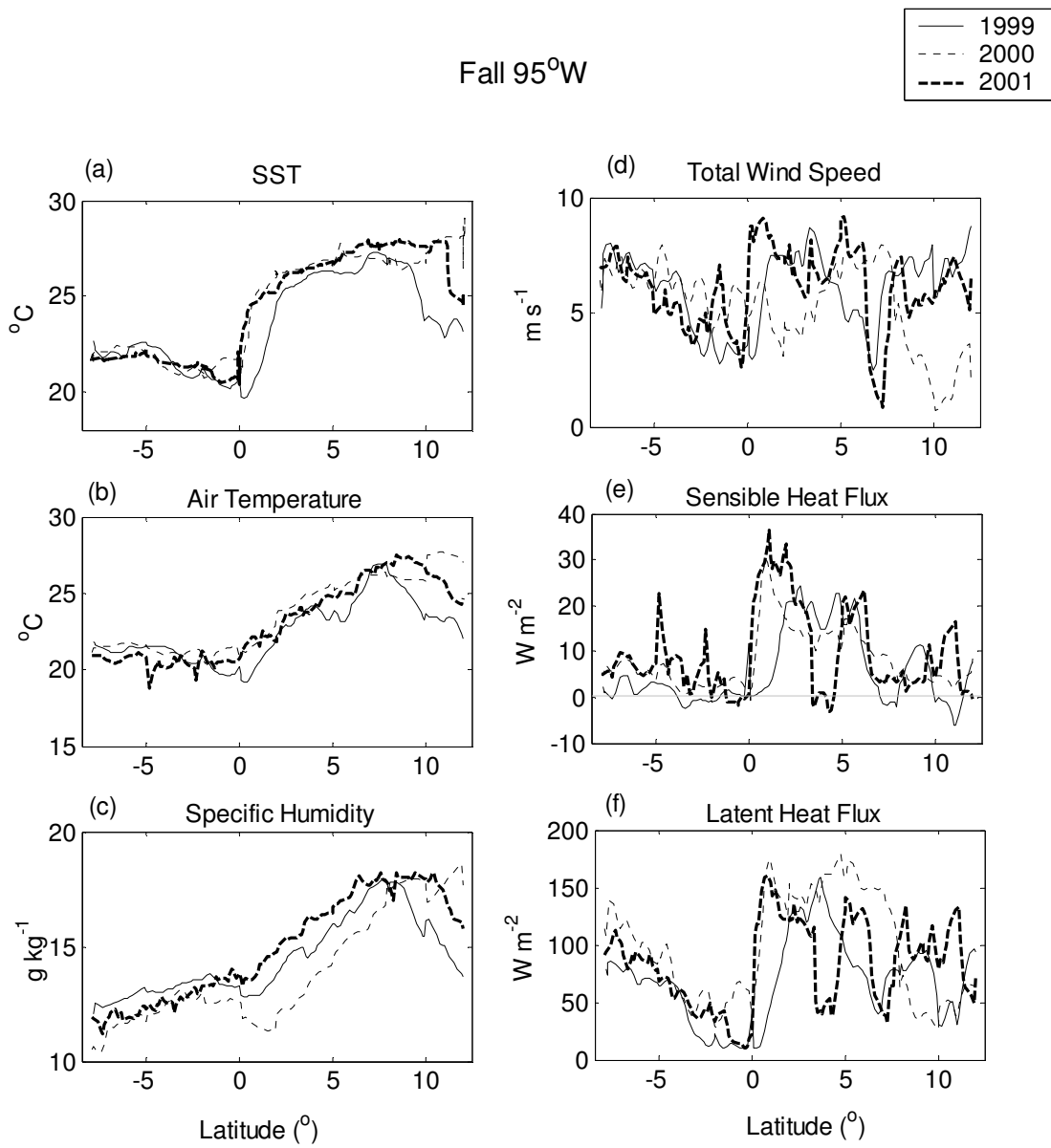
Figure 4 – Ship measurements for fall seasons 1999-2001.
