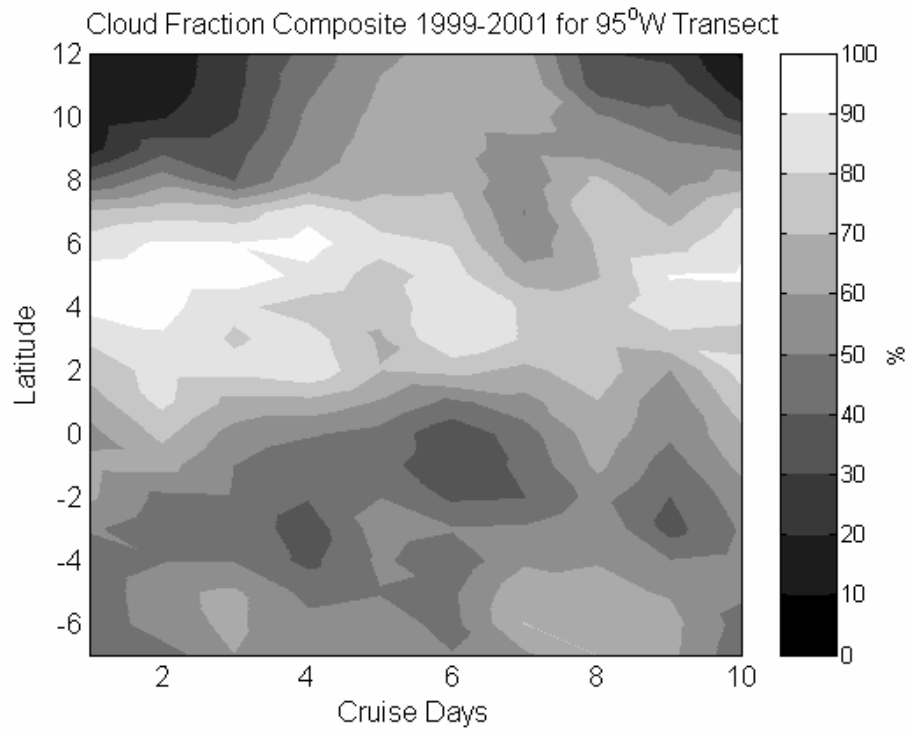
Figure 11—Satellite derived cloud fraction composite for 1999-2001.
