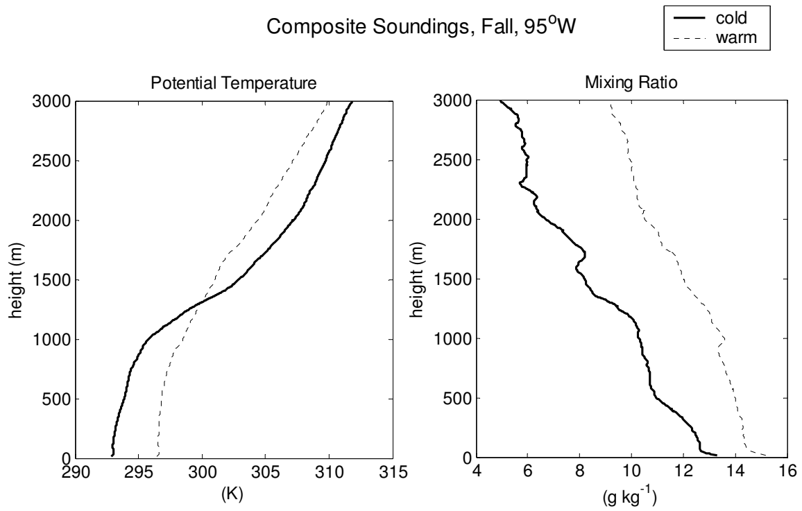
Figure 15 – Composite soundings for the cold (4°S-0°N) and warm (2°-6°N) sides of the SST gradient for the fall seasons from 1999-2001.
