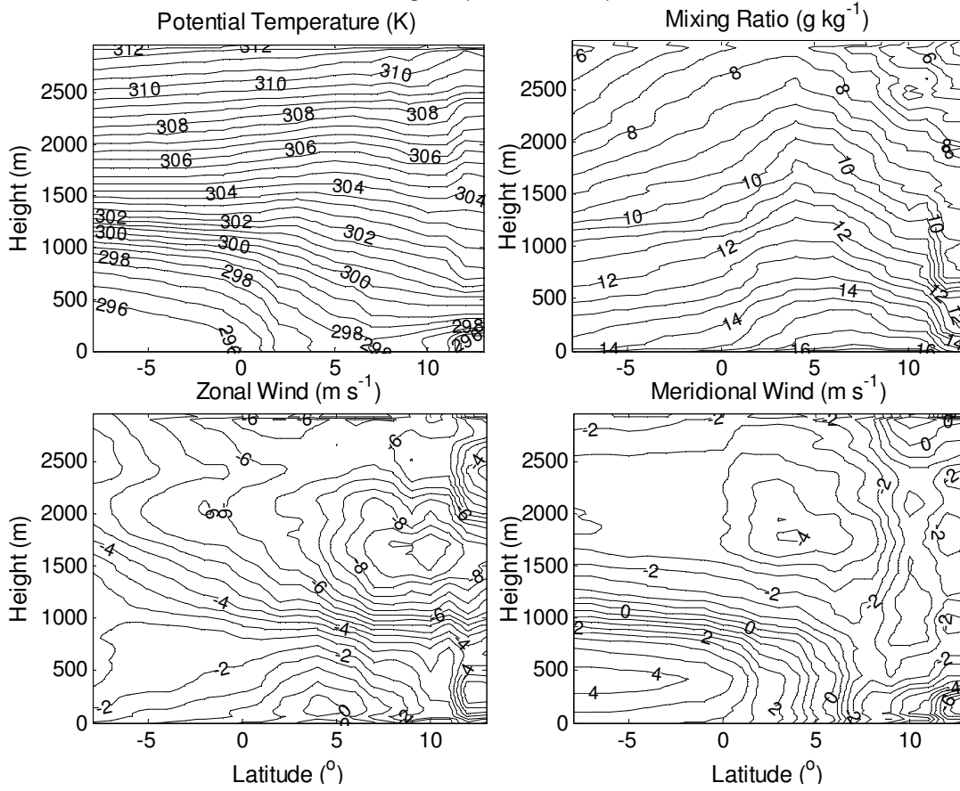
Figure 6 – North-south cross section of the average of fall seasons (1999-2001).
