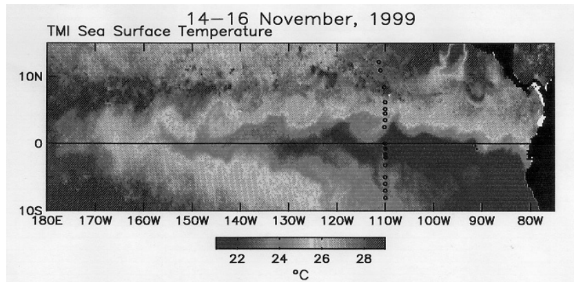
Figure 1—TMI Satellite measured SST. The dark area extending from the South American coast is the cold tongue. The undulations along the cold tongue are caused by westward propagating tropical instability waves. Circles indicate the cruise track along 110°W during November, 1999.
