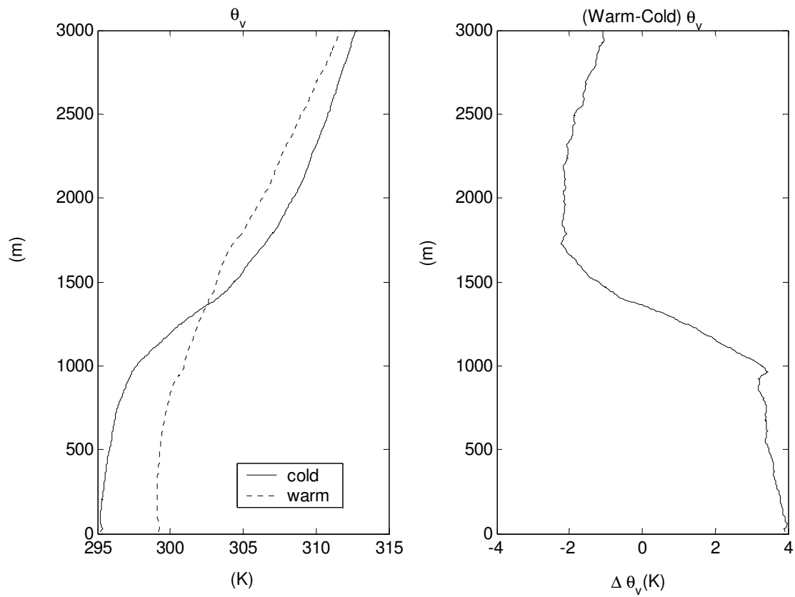
Figure 17—Composite (1999-2001) of virtual potential temperature on cold and warm sides of the equatorial front (left) and the warm minus cold difference of virtual potential temperature (right).
