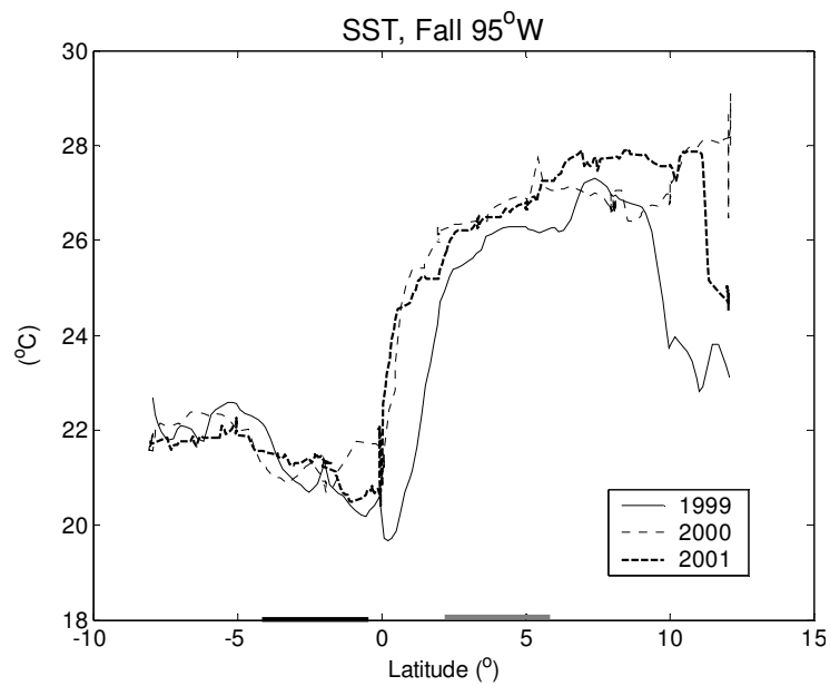
Figure 3 – SST vs. latitude for the fall cruises along 95°W. The black (cold) and gray (warm) horizontal lines along the x-axis indicate the latitudinal bands where soundings were grouped relative to the SST gradient for compositing.
