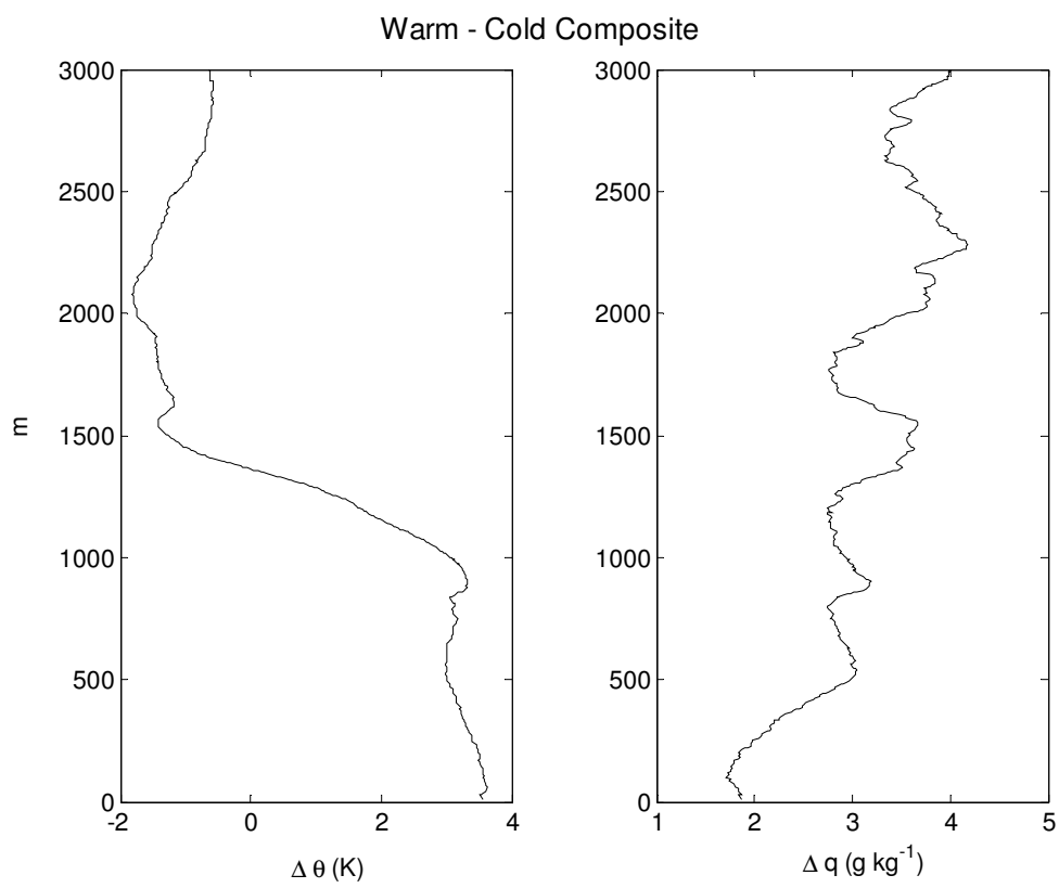
Figure 16 – Difference between warm and cold composites for composite of fall 1999-2001 seasons.
