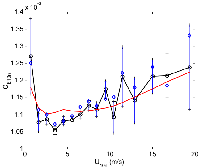
Fig. 4. Median moisture 10-m neutral transfer coefficient as a function of 10-m neutral wind. The diamonds are computed with method 1 (see text); the circles with method 3. Errors bars indicate the statistical uncertainty (one sigma) of the mean estimate based on the distribution within the wind speed bin. The heavy solid line is COARE 2.6
