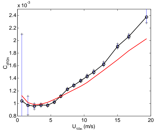
Fig. 5 Median 10-m neutral velocity transfer coefficient as a function of 10-m neutral wind. The circles are computed with 3. Errors bars indicate the statistical uncertainty (one sigma) of the mean estimate based on the distribution within the wind speed bin. The heavy solid line is COARE 2.6
