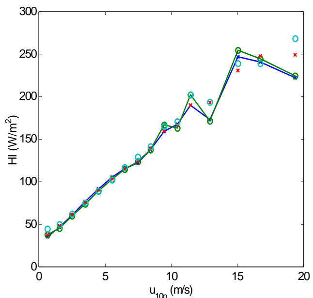
Fig. 1. Mean (line) and median (no line) fluxes computed in wind speed bins for 4272 selected hours of latent heat flux data. The x 's are COARE 2.6 values; the circles are the average of covariance and ID values.
