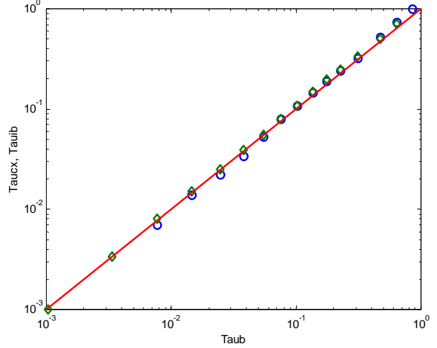
Fig. 3. As in Fig. 2 but for turbulent stress. The circles are the covariance values; the diamonds are the inertial-dissipation values. Negative covariances at very low winds are not shown.
