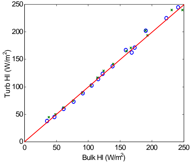
Fig. 2. The same data points from Fig. 1 but plotted as bulk latent heat flux values versus turbulent values. The x's are the means; the circles are medians.
