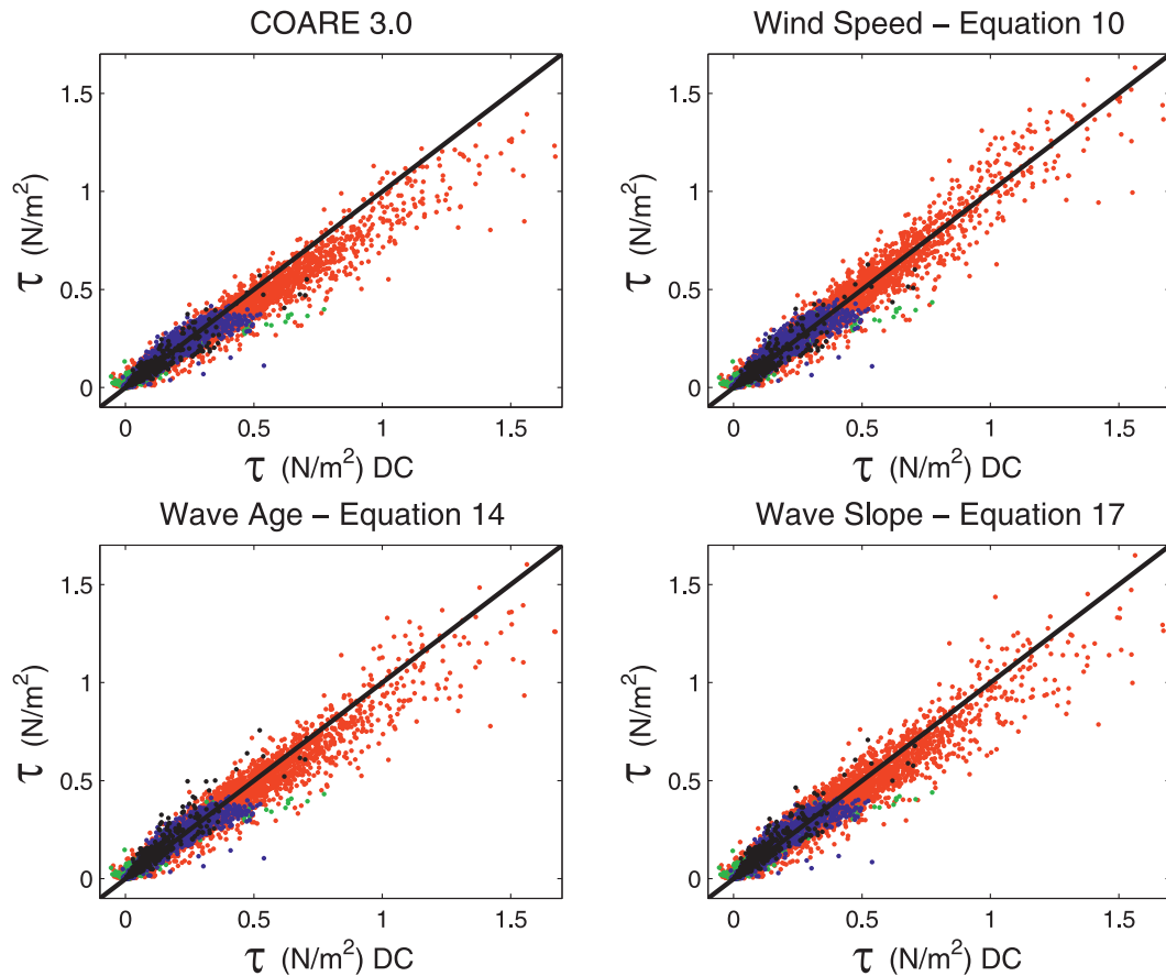
FIG. 11. Scatterplots of DC estimate of the surface stress vs (top) (left) the COARE 3.0 algorithm and (right) wind speed; and (bottom) (left) wave age, and (right) wave slope based parameterization developed in this study for COARE 3.5. The red points are from the CLIMODE buoy, the blue from MBL, the green from CBLAST, and the black from RASEX.
