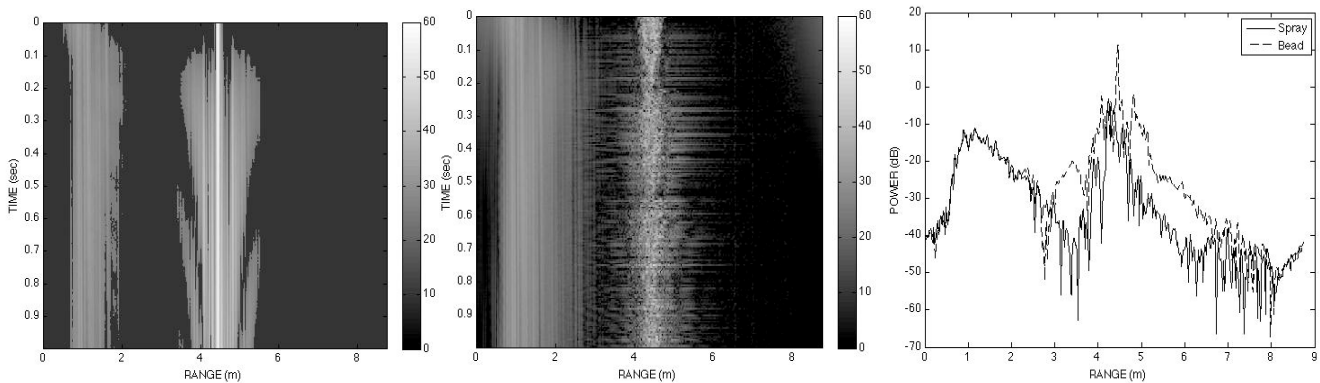
Figure 2. FMCW time-range images of a 3 mm gold bead (left) and water spray (center), in relative (uncalibrated) power in dB scale. At right is a horizontal cut through both left and center data, showing received power versus range.
