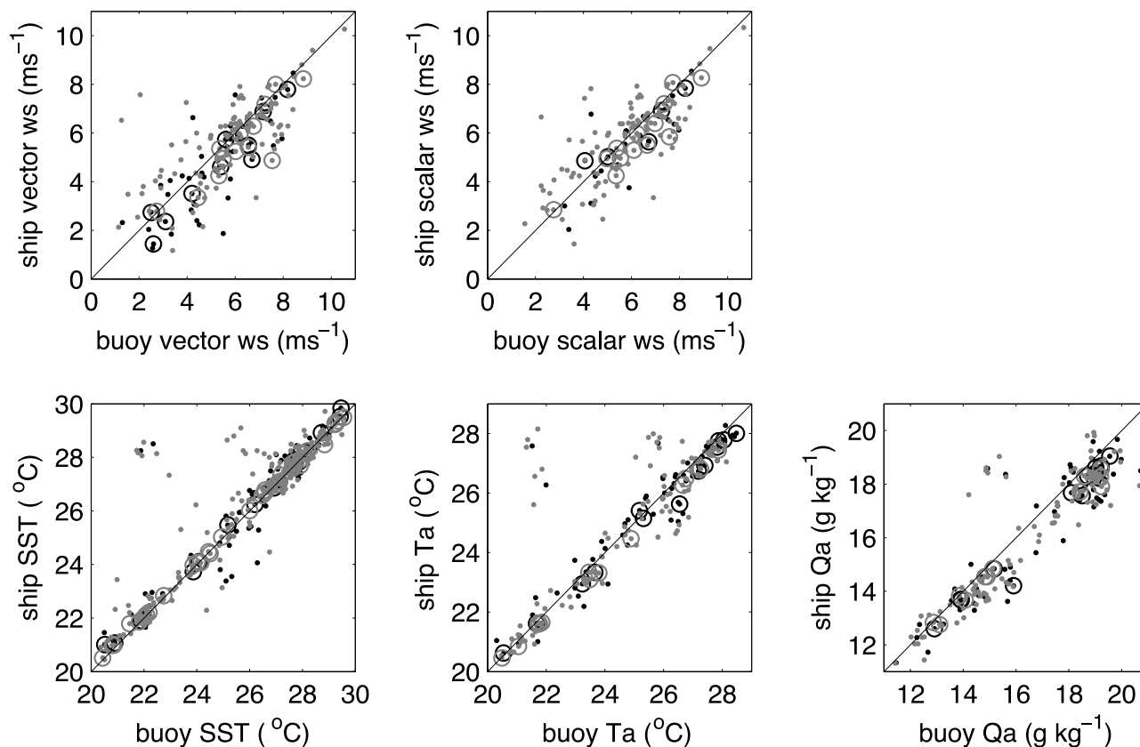
Figure 9. Scatterplots 24-hour-averaged (black) and 6-hour-averaged (gray) state variables from ship and buoys along 95°W and 110°W. Dots indicate measurements from the ship and the nearest buoy. Circles indicate that the ship and buoy were less than ~10 km apart at the center of the averaging interval.
