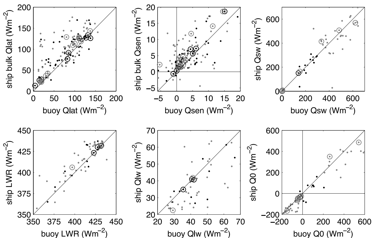
Figure 10. Same as Figure 9 but for surface heat flux measurements. Radiation buoy measurements were limited to 95^{\circ}W .
