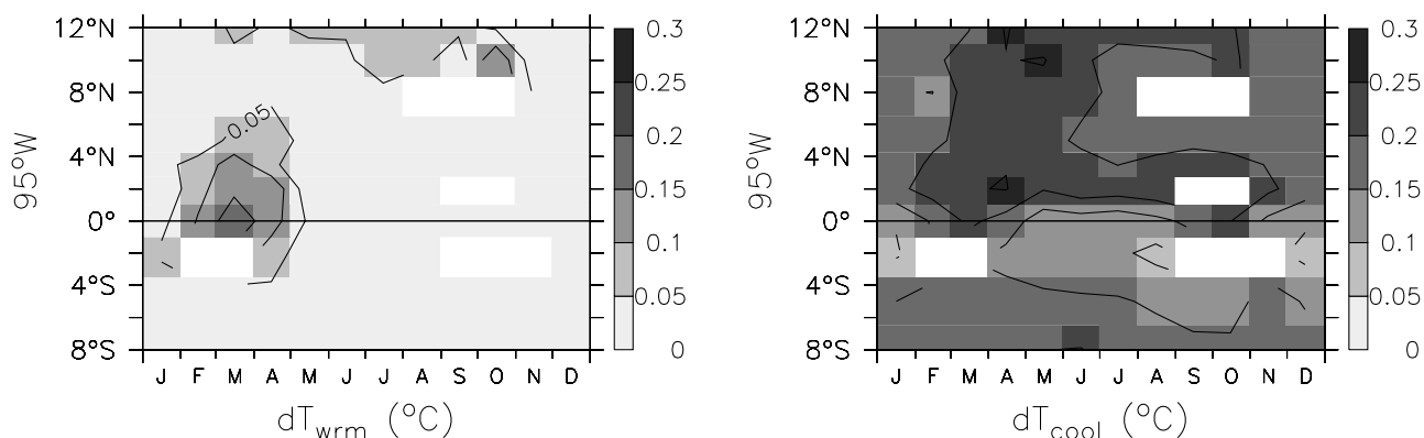
Figure 11. Annual cycle of the warm layer and cool skin temperature corrections along 95^{\circ}W as estimated from the Coupled Ocean Atmosphere and Response Experiment (COARE) v3.0 bulk algorithm.
