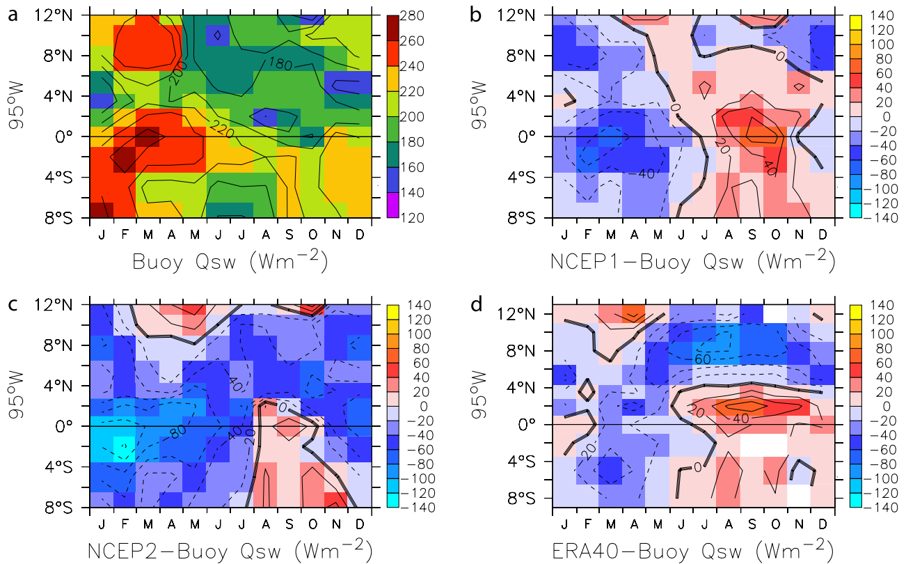
Figure 14. (a–d) Same as Figure 12 but for net solar radiation. A positive net solar radiation value indicates heat gained by ocean.
