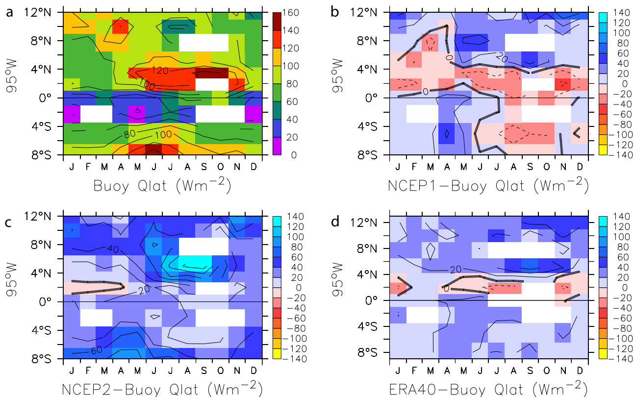
Figure 12. (a) Mean annual cycle of latent heat flux along 95°W from 8°S to 12°N from TAO/EPIC buoy measurements. (b) Mean annual cycle of difference between NWP and buoy latent heat flux field along 95°W from 8°S to 12°N for NCEP1. (c) Mean annual cycle of difference between NWP and buoy latent heat flux field along 95°W from 8°S to 12°N for NCEP2 reanalysis. (d) Mean annual cycle of difference between NWP and buoy latent heat flux field along 95°W from 8°S to 12°N for ERA40. A positive latent heat flux value indicates heat loss by ocean.
