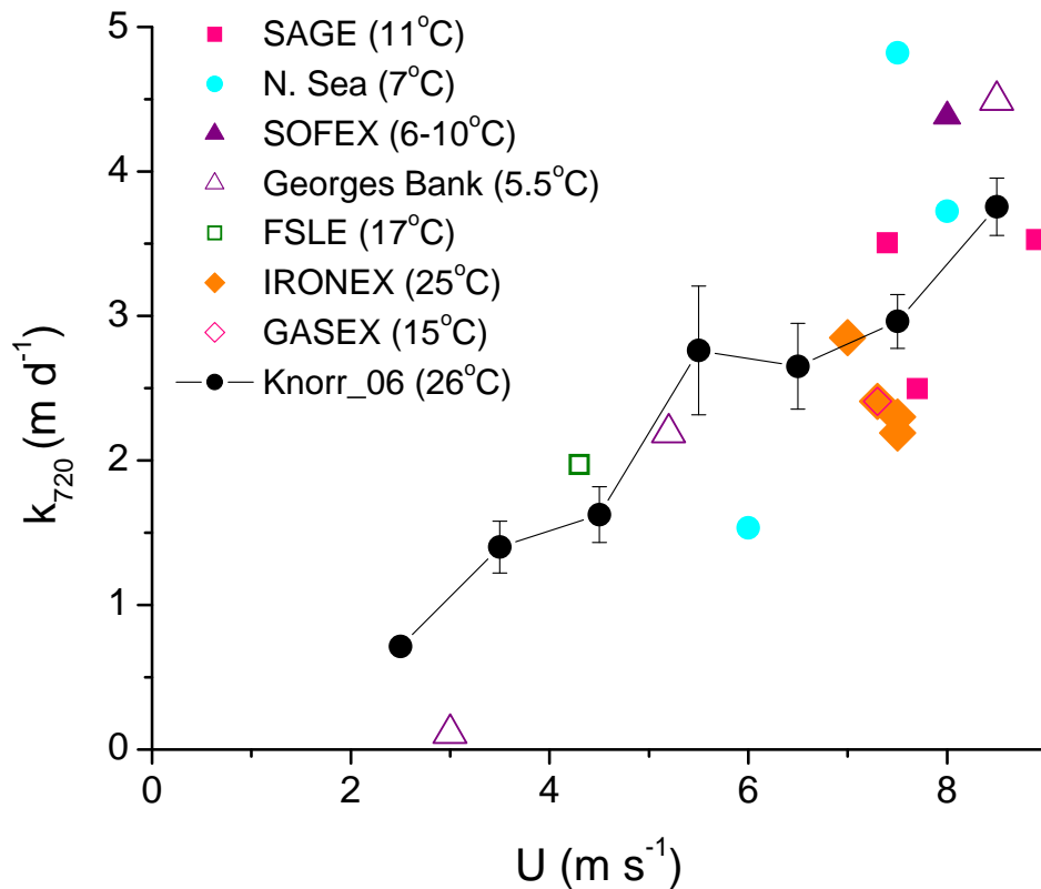
Figure 9. Comparison between k_{720} for DMS measured in this study and those measured by various dual tracer experiments. The Knorr_06 data has been binned by wind speed and error bars are the standard error of the mean. All the data has been normalized to a Sc=720 .
