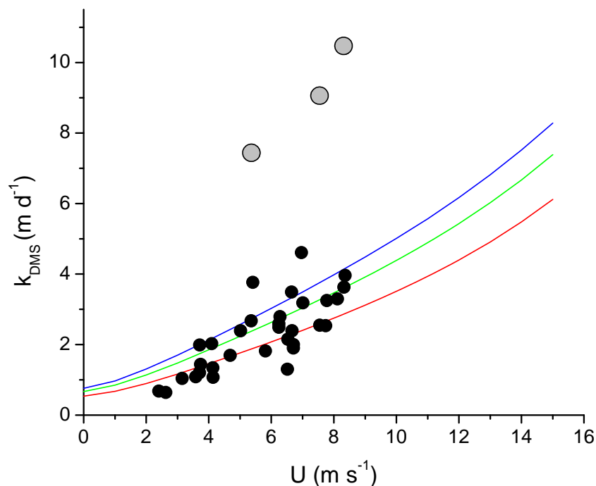
Figure 11. The wind speed dependence of the DMS gas transfer coefficient measured in Knorr_06 (closed circles) compared to various NOAA/COARE model runs with different tunable parameter A values ( A=2.0 , blue line; A=1.7 , green line; A=1.3 , red line).
