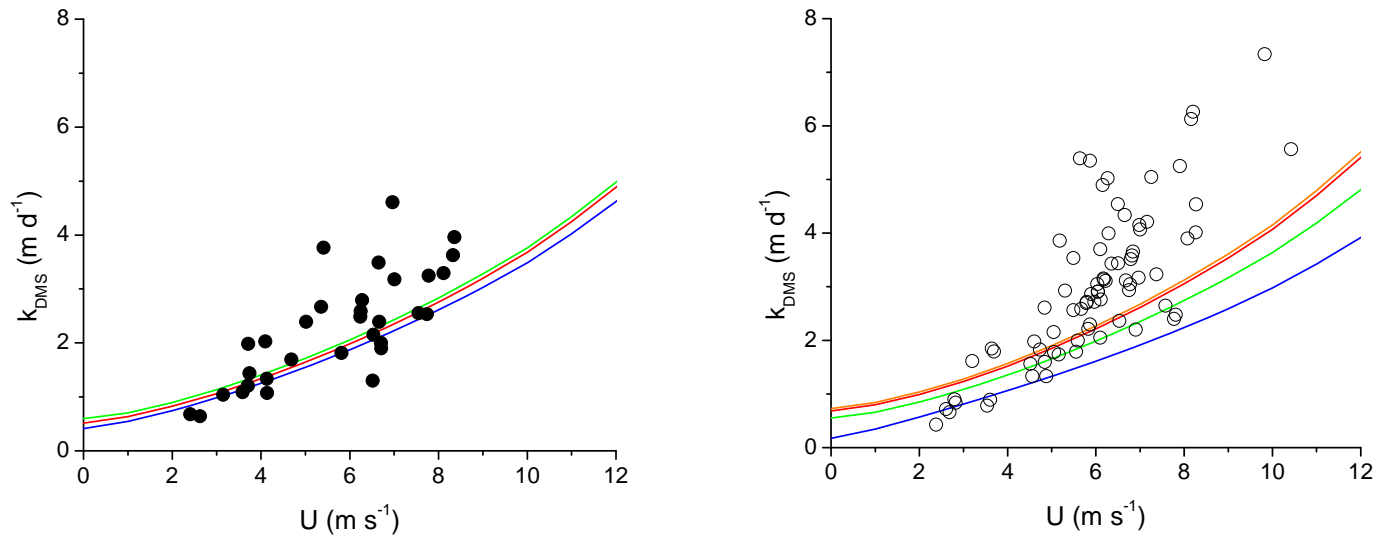
Figure 10. Modeled and measured wind speed dependence of the gas transfer coefficient using the NOAA-COARE model. Left panel - Knorr_06. The red, green, and blue lines represent modeled k values for the upwelling, gyre, and subpolar regions, respectively. Right panel - PHASE I cruise. The red, orange, green, and blue lines represent modeled k values for the warm pool, equatorial upwelling, gyre, and subpolar front regions, respectively. Solid black circles are measured k values from Knorr_06, open circles are PHASE I measured k values, and solid grey circles are the outliers discussed in the text. The k values are not normalized by Schmidt number. Modeled k values include bubble parameterization. Model tunable parameters were A=1.3 and B=1.0 .
