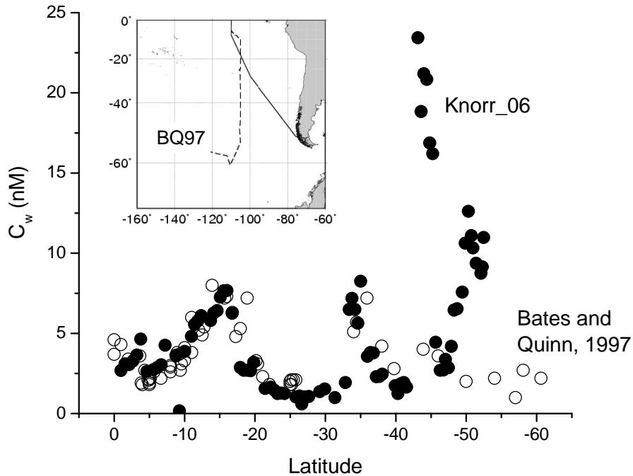
Figure 5. Latitudinal comparison of surface seawater DMS concentrations from Knorr_06 (closed circles) and Bates and Quinn (1997) (BQ97, open circles). The map inset depicts the cruise track from Knorr_06 (black line) and that from BQ97 (grey line).
