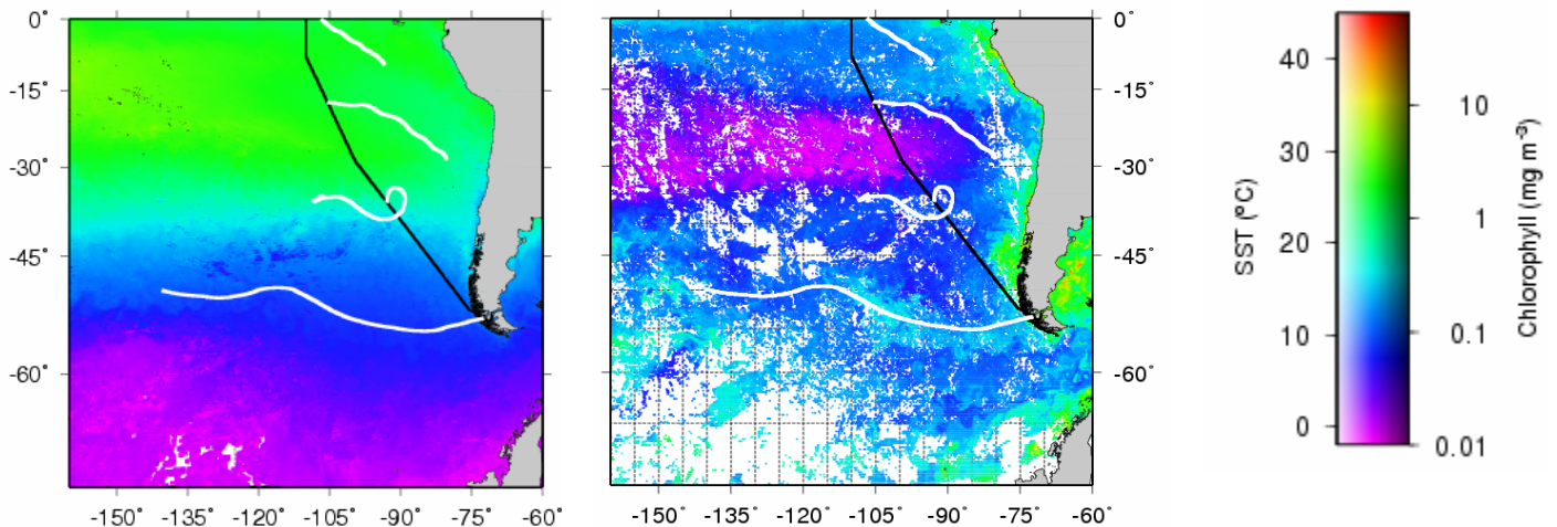
Figure 3. The cruise track superimposed on Modis data. Left panel - SST ( ^\circ \text{C} ). Right panel - chlorophyll ( \text{mg m}^{-3} ). Solid white lines are 5 day surface air mass back trajectories.
