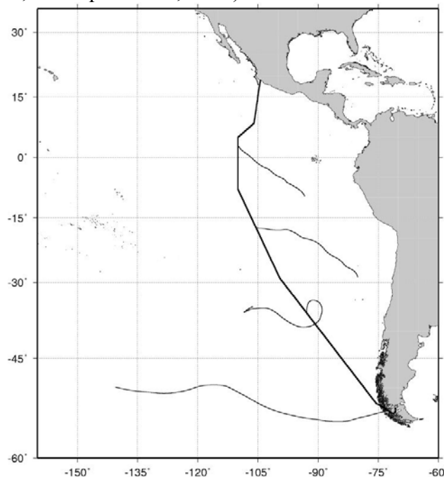
Figure 1. Cruise track for the Knorr_06. Solid grey lines are five day surface air mass back trajectories.
