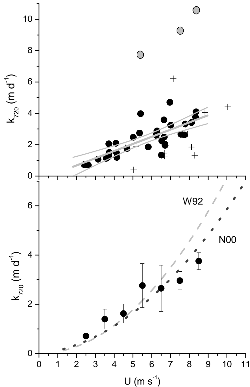
Figure 6. Wind speed dependence of computed gas transfer coefficient normalized to Sc=720 . Top panel - best quality 1-hour k values (closed circles) and lower quality k values (plus signs). The solid gray lines are a linear fit to the data with 95% confidence bands. Bottom panel - k values binned in 1 \text{ m s}^{-1} intervals. Error bars are \pm 1 s.e. Gas transfer parameterizations of Wanninkhof (1992; W92 dashed gray line), and Nightingale et al. (2000a; N00, dotted black line), normalized to Sc=720 are also shown. Gray closed circles indicate outlier points discussed in text.
