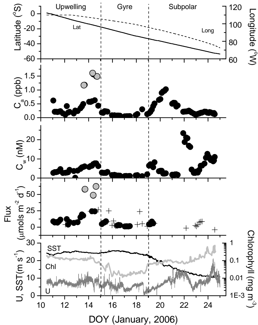
Figure 4. Time series of shipboard data. From top: a - Cruise track latitude (solid) and longitude (dashed), b - DMS atmospheric mixing ratio, c - DMS oceanic concentration, d - DMS air/sea flux, in which closed circle represent the highest quality data used to compute k and plus signs are other fluxes discussed in text, e - Sea surface temperature (solid black), and chlorophyll concentration (solid grey). The vertical dashed lines indicate the upwelling, gyre, and subpolar front regions of the cruise. Grey closed circles indicate outlier points discussed in text.
