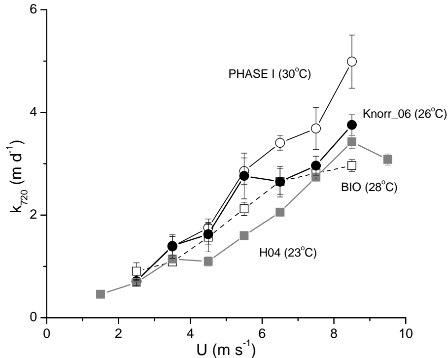
Figure 7. Wind speed dependence of computed gas transfer coefficients from this work (solid black circles), the PHASE I (open circles) cruise, H04 (grey closed squares), and the BIO cruise (open squares), normalized to Sc=720 . All cruises binned by wind speed. Error bars represent the standard error of the mean (if error bars are not visible they are the size of the symbol).
