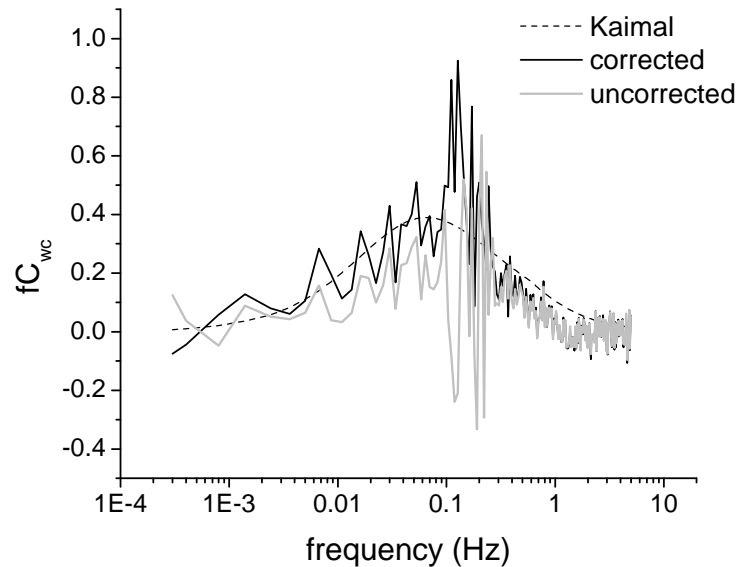
Figure 2. DMS w frequency weighted cospectra from the morning of 11 January 2006. The solid black line is the cospectrum corrected for ship motion, solid grey is the motion uncorrected cospectrum, and the dashed line is the idealized scalar cospectrum from Kaimal et al. (1972).
