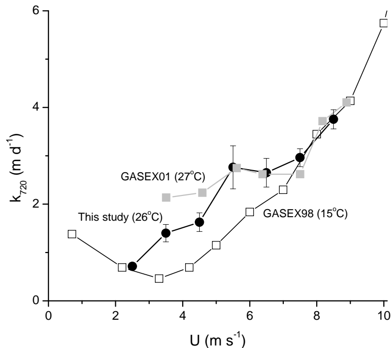
Figure 8. Wind speed dependence of computed gas transfer coefficients from this work (solid black circles), the GASEX 1998 (McGillis et al., 2001) cruise (open squares), and the GASEX 2001 (McGillis et al., 2004) cruise (grey closed squares), normalized to Sc=720 . Error bars represent \pm 1 s.e..
