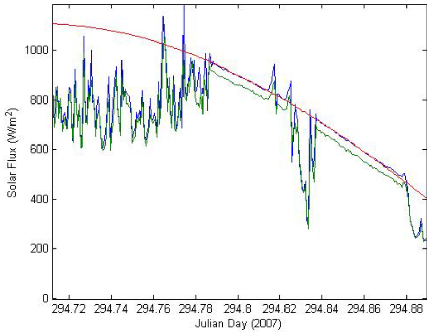
Figure 1. Solar flux vs time at 1-min resolution on from the WHOI flux reference site at 20 S 85 W Julian Day 294: red line – clear sky flux model; blue line – mean of two K&Z sensors; green line - mean of five Eppley sensors. The lower panel is a detail from JD 294.71 to JD 294.89 (4.3 hrs). Clear periods are indicated by very smooth traces of the time series and values near the clear-sky flux model (e.g., between 294.78 and 294.82). Note the green line is about 3% lower than the blue line.
