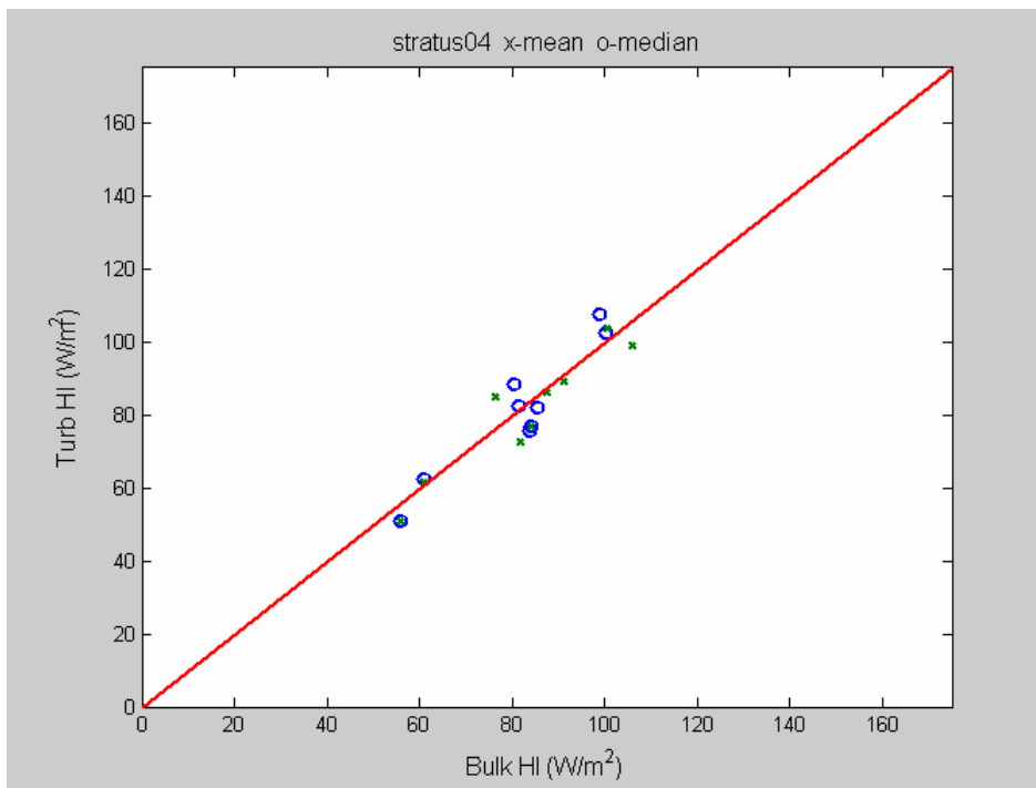
Figure 31. Average bulk latent heat flux vs direct values from wind speed bins (0 – 1 m/s) for the Stratus04 cruise: x-mean and o-median.
