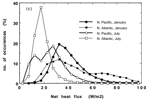
Fig. 3. Histograms of the interannual variability of monthly 1^\circ \times 1^\circ mean values of the net heat flux for the North Atlantic and North Pacific oceans for January and July as calculated from the SOC surface flux climatology (Josey et al. 1999)
