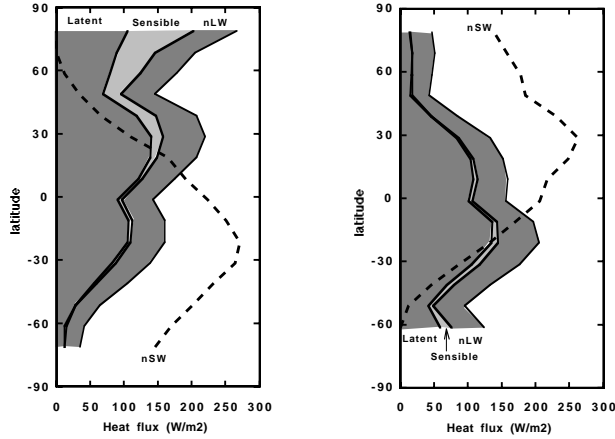
Fig. 2. Zonal mean values of the flux components derived from the SOC climatology (Josey et al. 1999) for (a) January; (b) July.
