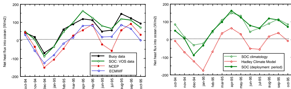
Fig. 5. Net heat flux at an Arabian Sea buoy site (adapted from Weller et al. 1997). Left: the measured buoy values, the values from the SOC flux dataset, and fluxes from the ECMWF and NCEP NWP models. In each case the data are for the actual buoy deployment period. Right: The SOC flux values for the deployment period and for the 1980 to 1993 mean values. Also shown are the fluxes from an AMIP run of the Hadley Centre climate model (Hall et al. 1995).
