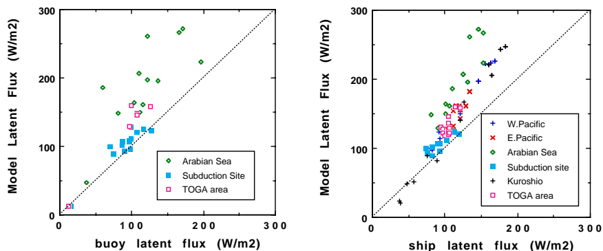
Fig. 8. Comparison of monthly mean latent heat fluxes from a model (the Hadley Centre HADAM3 model) and (left) estimates from IMET buoy deployments; (right) values from the SOC ship-based climatology.
