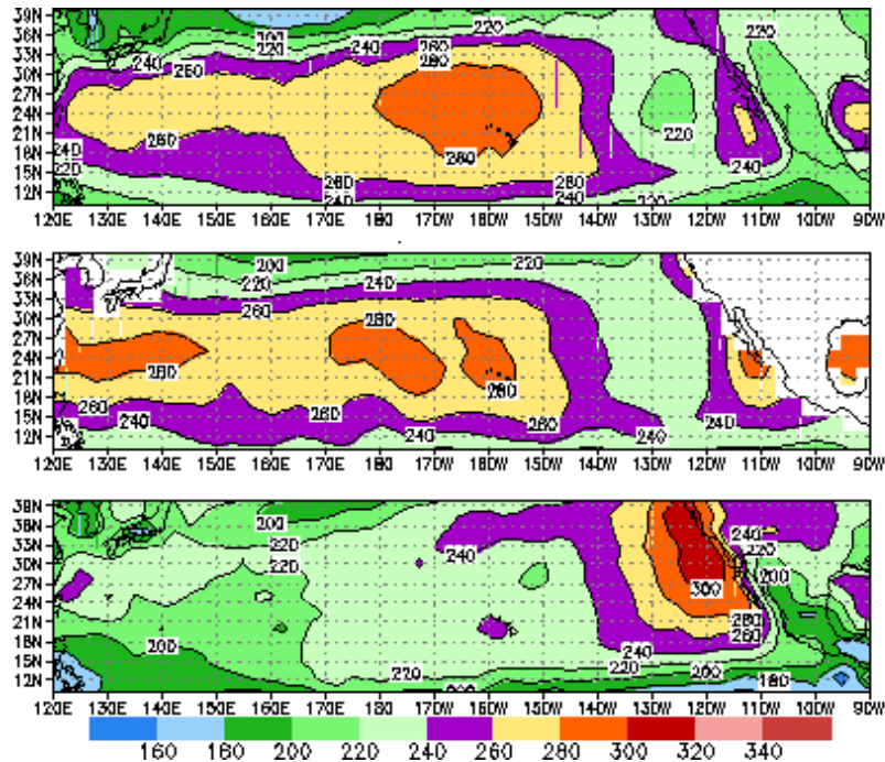
Fig. 6. Net shortwave radiation at the ocean surface for July 1983-1990: (top) satellite based estimate (Darnell et al. 1992); (middle) ship based estimate (da Silva et al. 1994) untuned; (bottom) ECMWF reanalysis (adapted from White & da Silva, 1999).
