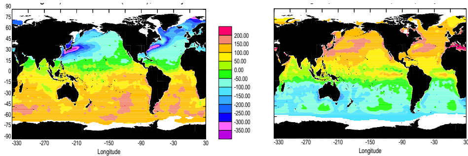
Fig. 1 Mean net heat flux from the SOC climatology (Josey et al. 1999): (left) January; (right) July.
