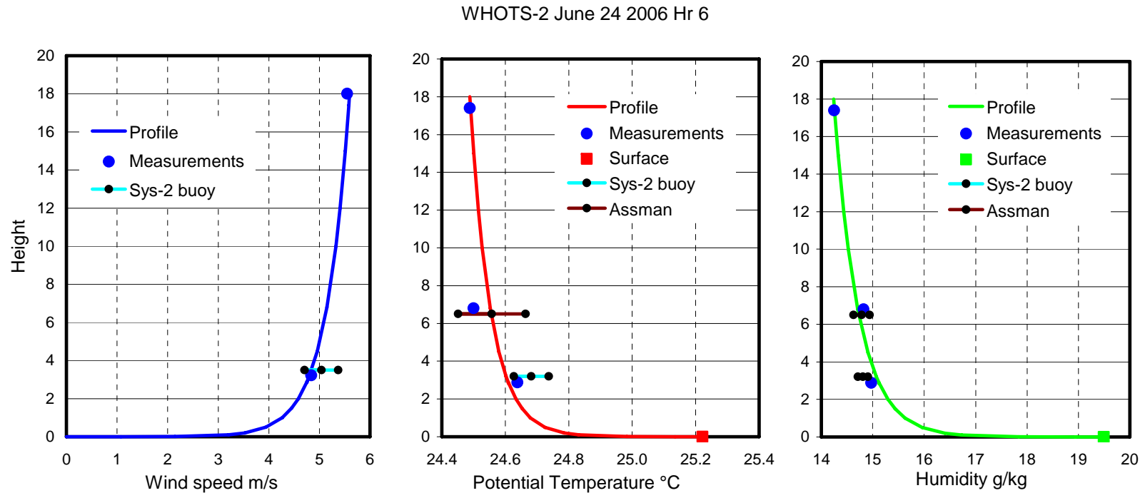
Figure A1. (Data courtesy Bob Weller). Example of need for height adjustment when comparing measured values at various levels above the sea surface. The ship’s anemometer was at 18 m on the foremast, and the temperature/humidity sensor at 17.4 m. Temperature and humidity were measured with an Assman psychrometer through a forward chock at 6.8 m height (see Figure 3.1). The ship was standing about 0.25 nm downwind of the WHOI buoy, which had two wind sensors at 3.22 m above the sea surface and two temperature/humidity sensors at 2.88 m. The ship and buoy data points are hourly averages; the Assman values are spot readings. The profiles were constructed from flux/gradient parameters calculated using Version 3.0 of the COARE bulk flux algorithm, and used in equation (11.7), as follows;
