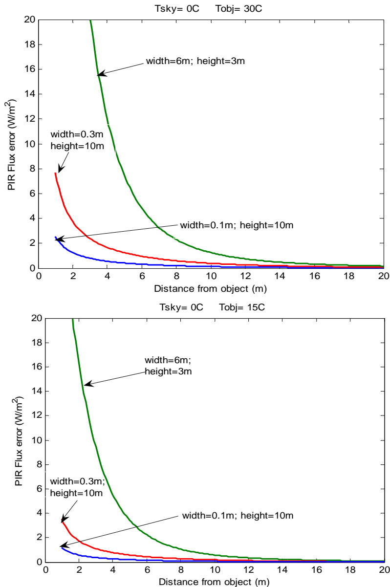
Figure C1. Longwave flux errors caused by shipboard objects in the field of view of a pyrgeometer; a tubular pole (blue), a mast (red), and a bulkhead (green). The assumed radiative sky temperature of 0°C is typical of mid-latitude clear-sky conditions. The lower panel is for an object at roughly ambient temperature; the upper panel is for an object warmed considerably by strong sunlight.
