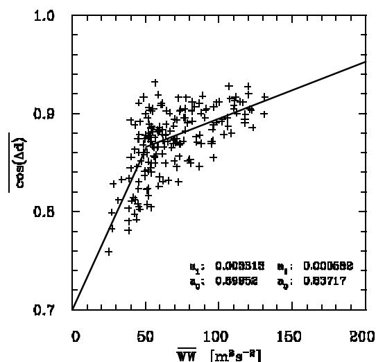
Figure 10.7 Relative error of the wind direction as a function of squared wind speed \overline{WW} . Individual crosses depict monthly 5^\circ x 10^\circ averages.
