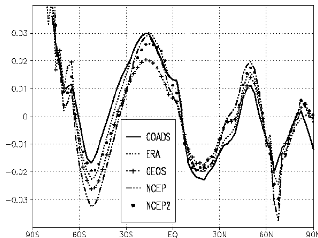
Figure 11.4.32 Zonally averaged meridional surface stress over the ocean averaged over 1981-92 from UWM and the reanalyses in \text{Nm}^{-2} .
