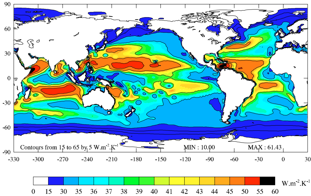
Figure 2.1: Sensitivity term \partial Q_{NS}/\partial SST ( \text{Wm}^{-2}\text{K}^{-1} ) estimated with atmospheric surface variables of the ECMWF re-analysis using the first order Taylor expansion of the bulk formulas proposed by Barnier et al. (1995).
