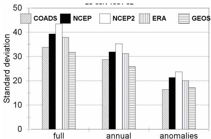
Figure 11.4.7(a) Standard deviation averaged over 20-60N of monthly mean latent heat release over the ocean in Wm^{-2} . Full values calculated from monthly means for 1981-92, annual from climatological monthly mean annual cycles averaged over 1981-92, and anomalies from departures of monthly means from the climatological annual cycle.
