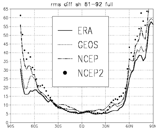
Figure 11.4.11(a) RMS differences in monthly mean sensible heat flux over the oceans between the reanalyses and UWM for 1981-92 in Wm^{-2} .
