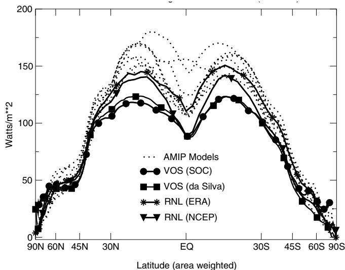
Figure 2.3 Zonal averages of the Global Ocean latent heat flux from reanalyses, observations (COADS) and AMIP2 (1998-99)
