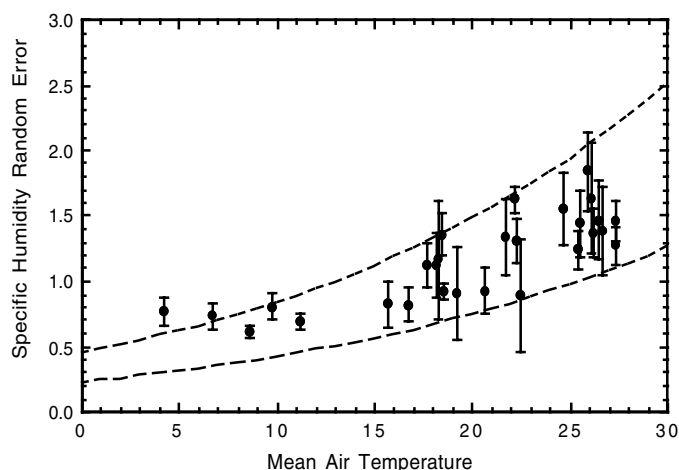
Figure 10.5. Random observational error in specific humidity ( \text{gkg}^{-1} ) as a function of mean air temperature ( ^{\circ}\text{C} ). The upper line is the error in specific humidity arising from a 2°C error in dew point temperature and the lower that from a 1°C error in dew point. A relative humidity of 80% has been assumed in the calculation. (from Kent et al. 1999)
