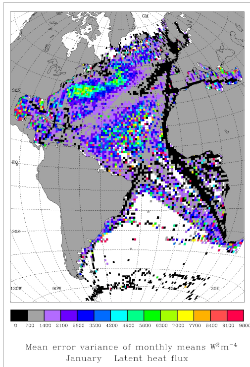
Figure 8.4. Error variance of monthly mean.
