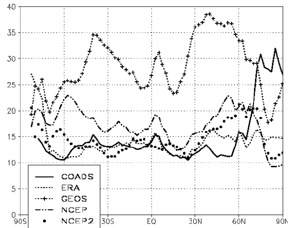
Figure 11.4.21(a) RMS differences in monthly mean surface NLW over the ocean of the reanalyses and COADS from SRB for July 1983-June 1991 in Wm^{-2} .
