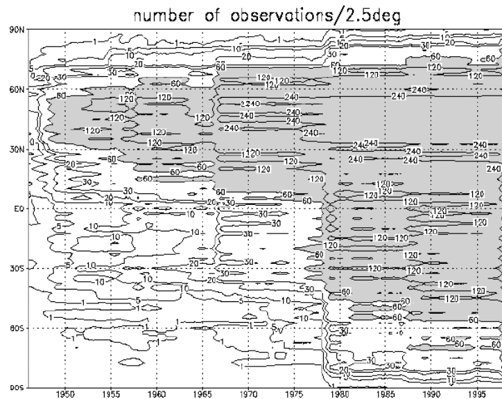
Figure 4.4. Zonally averaged number of all types of observations available to the NCEP/NCAR reanalysis per 2.5° latitude-longitude box per month from 1946 to 1998. A twelve-month running mean has been applied. Shading indicates more than sixty observations per month.
