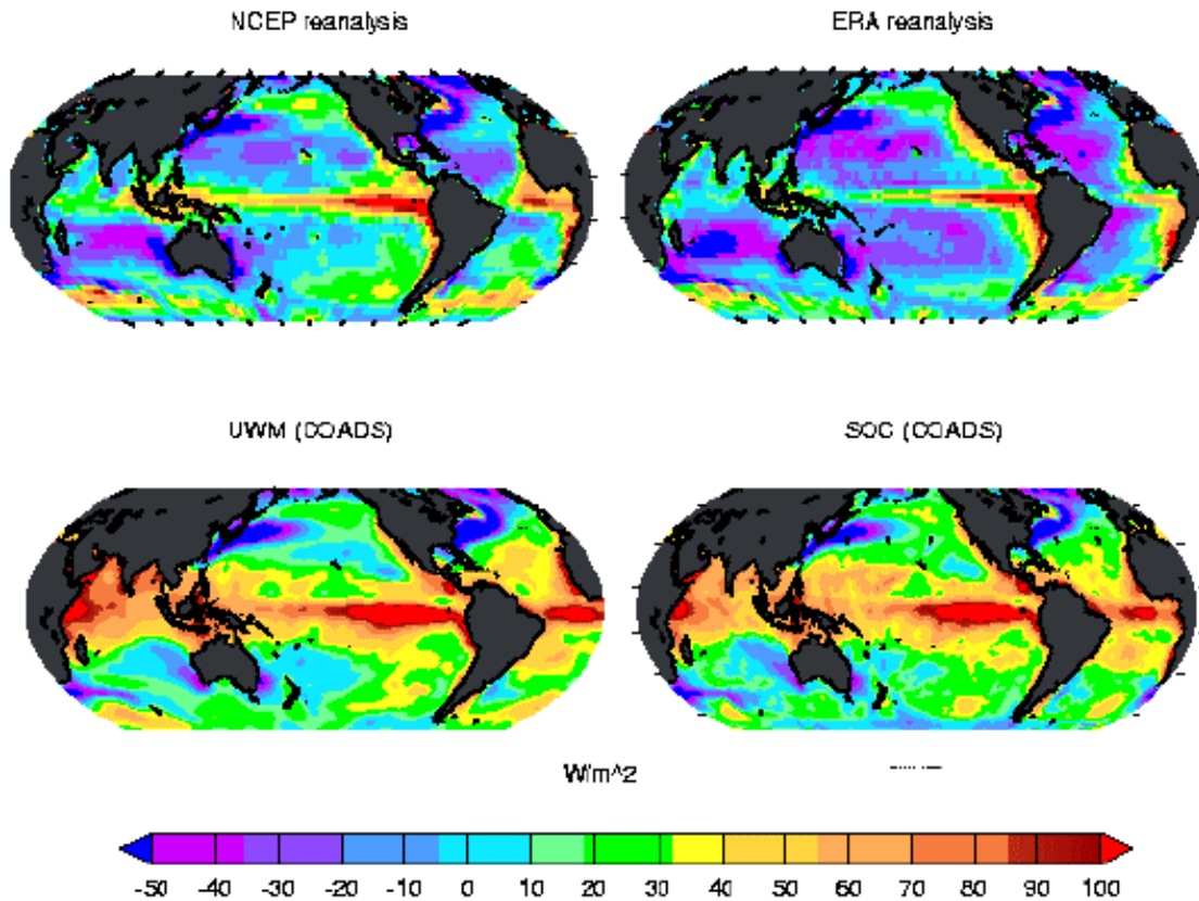
Figure 1.1 The climatological annual mean net surface heat flux from the atmosphere into the ocean (negative implies ocean cooling). Shown as examples are values from the NCEP/NCAR reanalysis, the ECMWF reanalysis, and the climatologies based on ship data in the COADS data set as calculated by UWM and SOC (see Chapter 11 for a detailed discussion)
