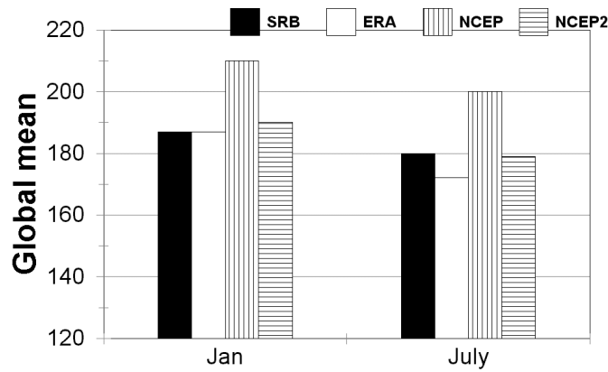
Figure 11.4.15 Global mean downward short wave radiation at the surface from SRB and from ERA, NCEP1 and NCEP2 reanalyses for Jan. 1984-91 and July 1983-90 in Wm^{-2} .
