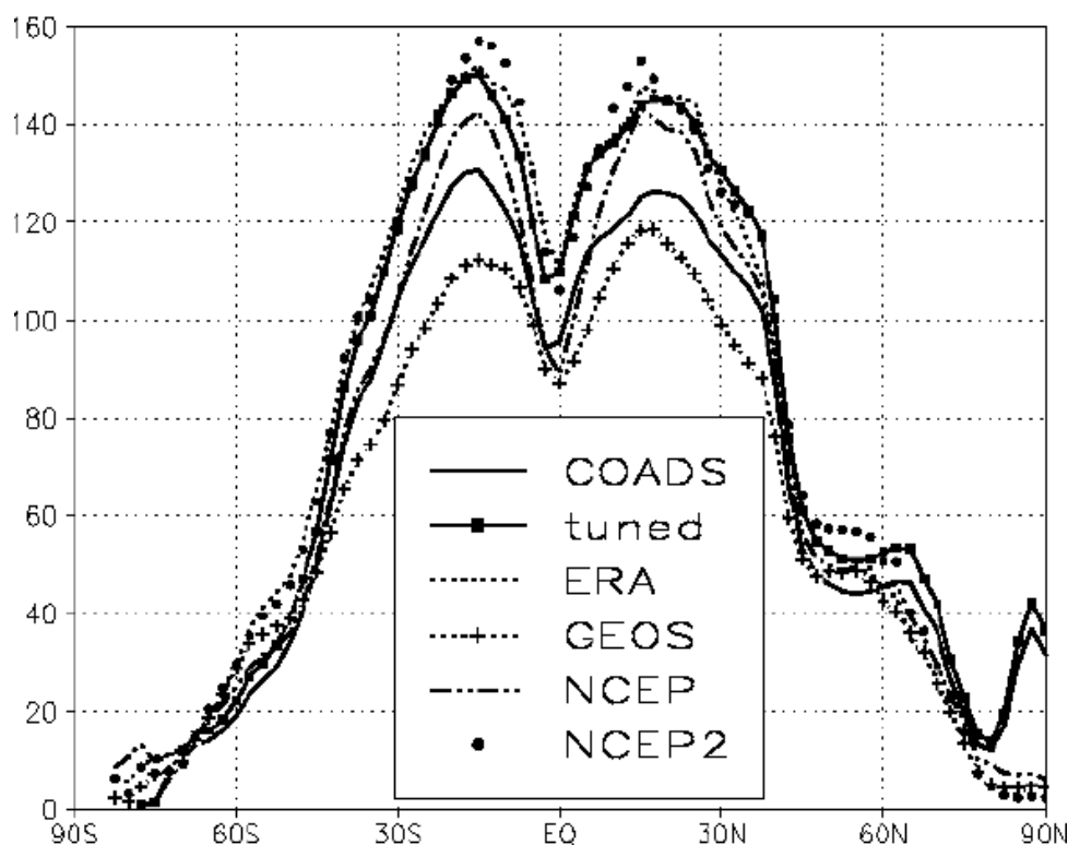
Figure 11.4.1 Zonal mean latent heat flux over the oceans for 1981-92 in Wm^2 .
