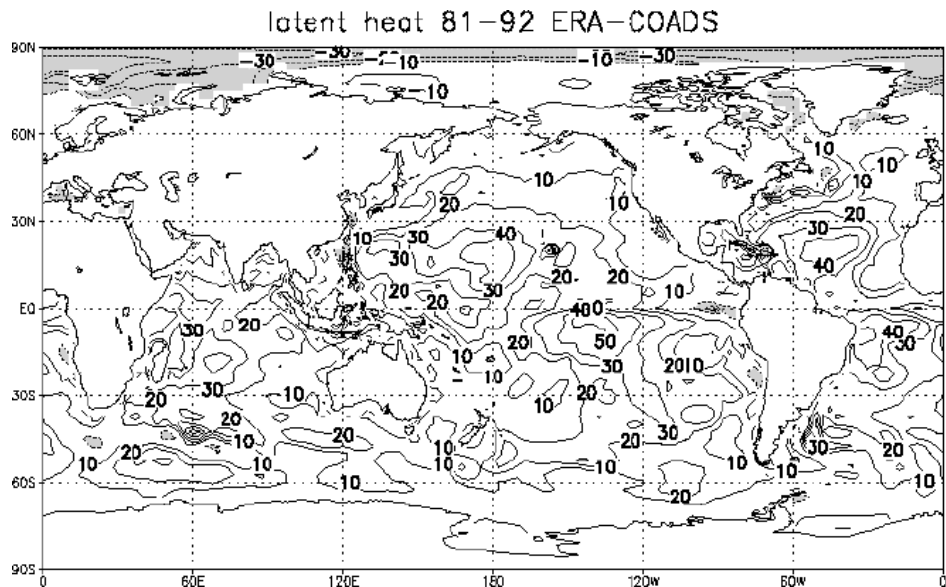
Figure 11.4.2: (a) Latent heat flux from the original COADS estimate (UWM) by da Silva et al. (1994) averaged over 1981-92. Contour interval 20 \text{ Wm}^{-2} , negative values shaded (b) Difference in latent heat flux ERA15 minus UWM averaged over 1981-92. Contour interval 10 \text{ Wm}^{-2} , zero omitted, negative values shaded. (c) As (b) but for GEOS1 minus UWM. (d) As (b) but for NCEP1 minus UWM. (e) As (b) but for NCEP2 minus UWM.
