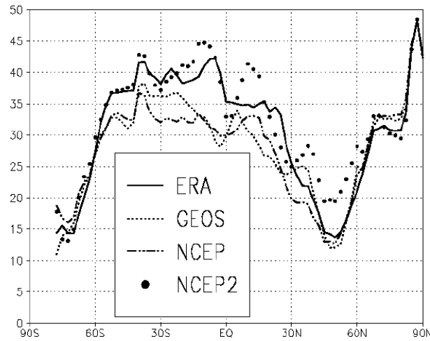
Figure 11.4.6a. Zonal mean root-mean square (RMS) difference in monthly mean latent heat flux over the oceans between the reanalyses and UWM for 1981-92 in Wm^{-2} .
