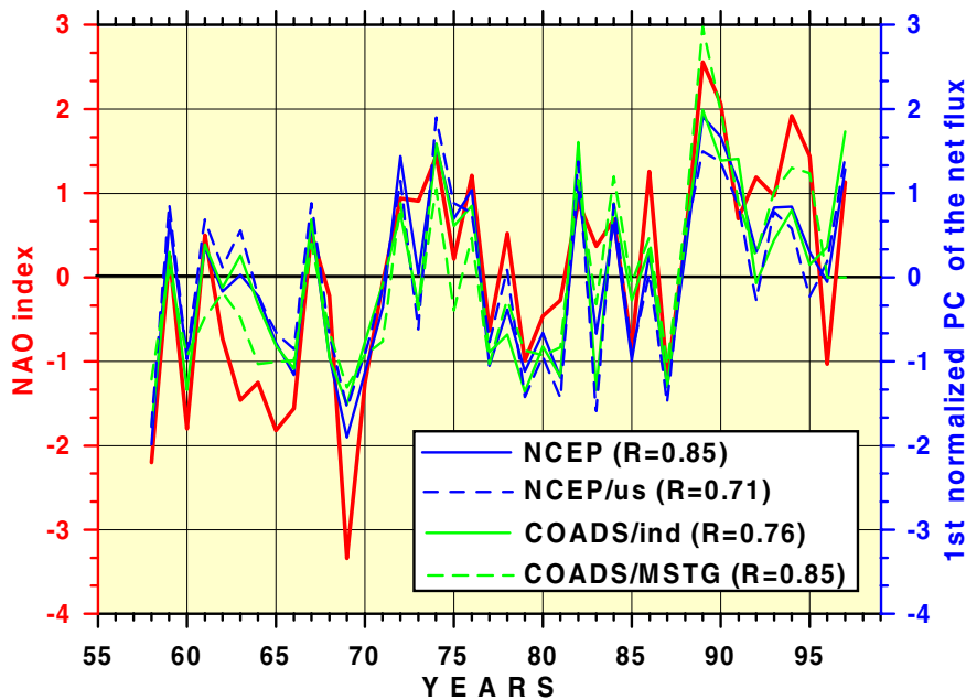
Figure 3.2 Time series of the NAO index (red line) and of the first normalised principal component of the net heat flux from the analyses shown in Figure 3.1. (NCEP/NCAR reanalysis; NCEP/us is sampled at ship data positions; Individual COADS reports; and COADS MSTG data.)
