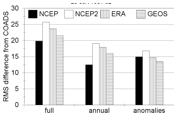
Figure 11.4.7(b) RMS difference averaged over 20-60N of monthly mean latent heat in the reanalyses from UWM in Wm^{-2} .
