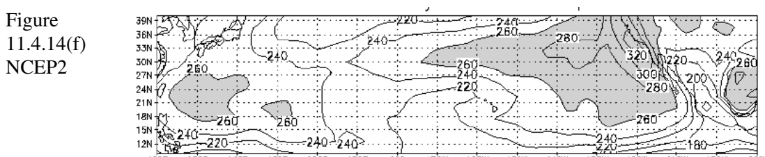
Figure 11.4.14. Surface NSW radiation from different sources averaged over July 1983-1990. Contour interval 20 \text{ Wm}^{-2} . Values over 260 \text{ Wm}^{-2} are shaded.
