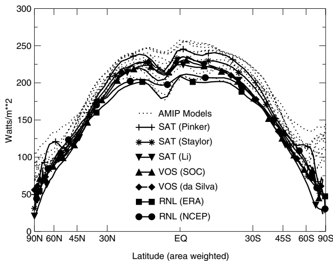
Figure 2.2 Zonal averages of the Global Ocean net SW flux from reanalyses, observations (COADS and satellites) and AMIP2 (1998-99)
