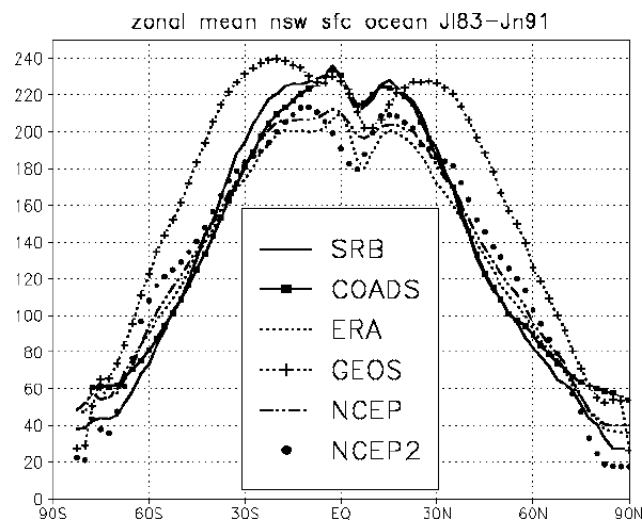
Figure 11.4.12 Zonal mean surface net short wave radiation over the oceans for 1981-92 in Wm^{-2} .
