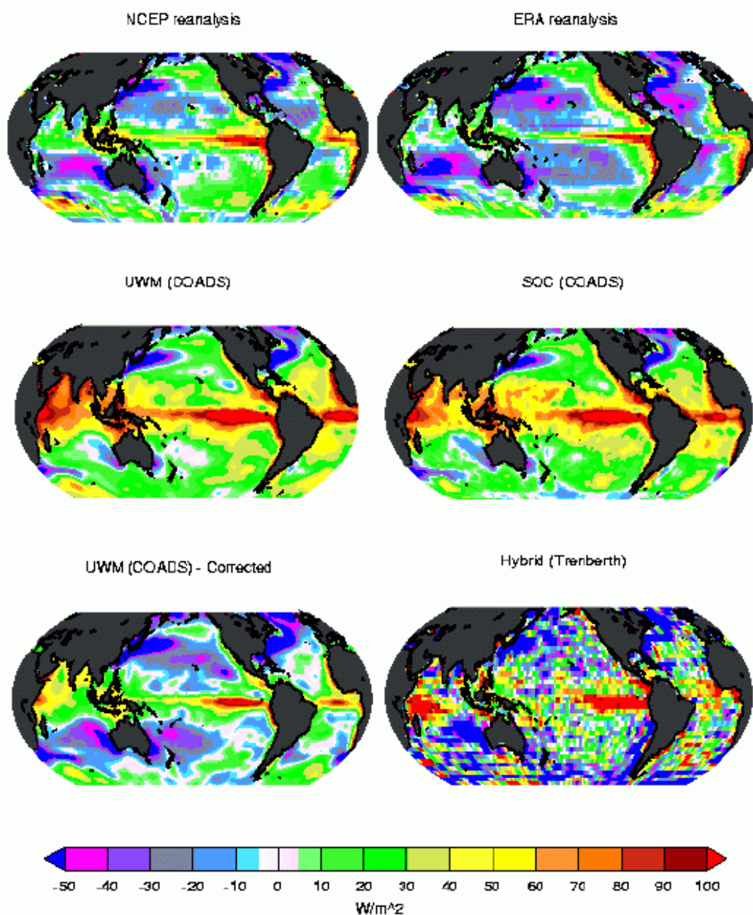
Figure 11.8.2 The annual mean climatology of six estimates of surface net heat flux. Shown are values from the NCEP reanalysis (top left), the ERA15 reanalysis (top right), the untuned UWM/COADS climatology (middle left), the SOC climatology (middle right), the tuned UWM/COADS climatology (bottom left), and the Residual method (Trenberth and Solomon, 1994) (bottom right).
