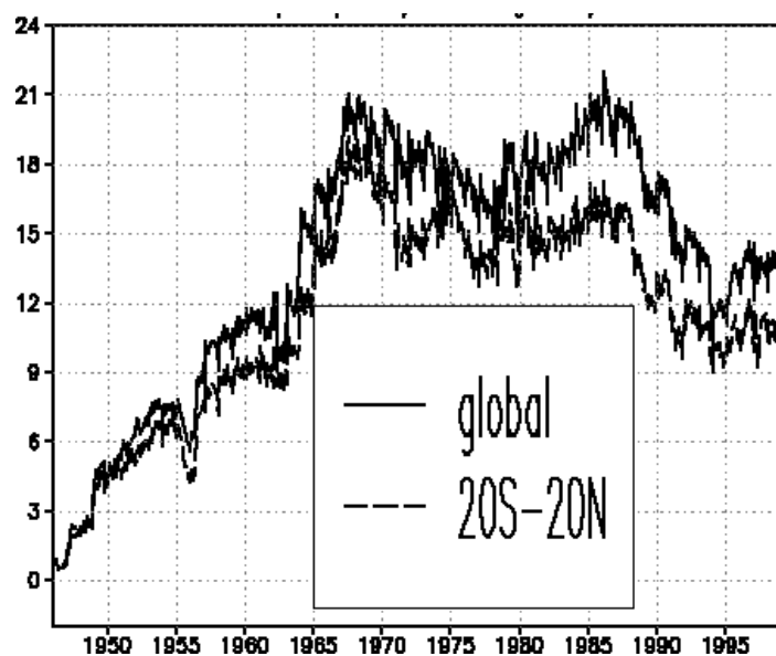
Figure 4.5: Zonally averaged number of ship reports per 2.5° box per month. Oceanic buoys are included.
