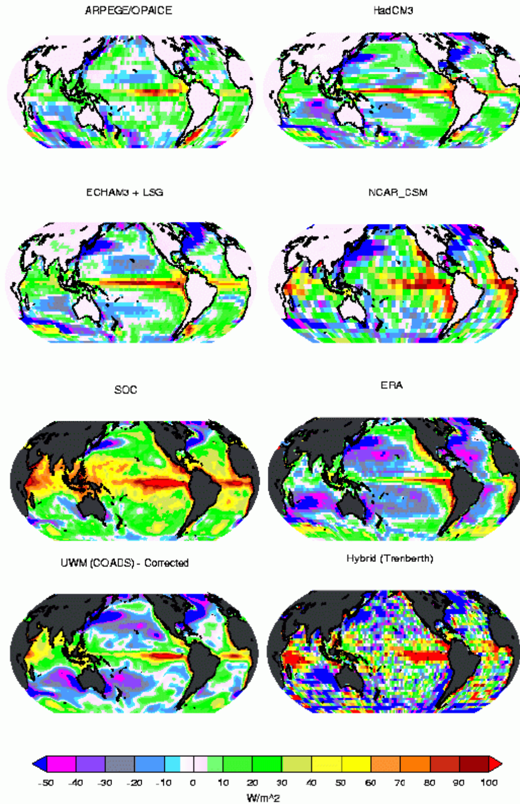
Figure 2.4. The climatological values of the net surface heat flux from four coupled models and four other flux products. Shown are (from top, left) ARPEGE/OPAICE, HadCM3, ECHAM3 + LSG, NCAR-CSM, the SOC climatology, the ERA15 reanalysis, the tuned UWM/COADS climatology, and the results from the Residual method (Trenberth and Solomon, 1994)
