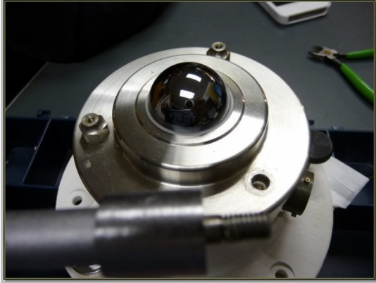
CW from top Left: Eppley Pyrgometer replacement dome (to go with body shipped previously)
