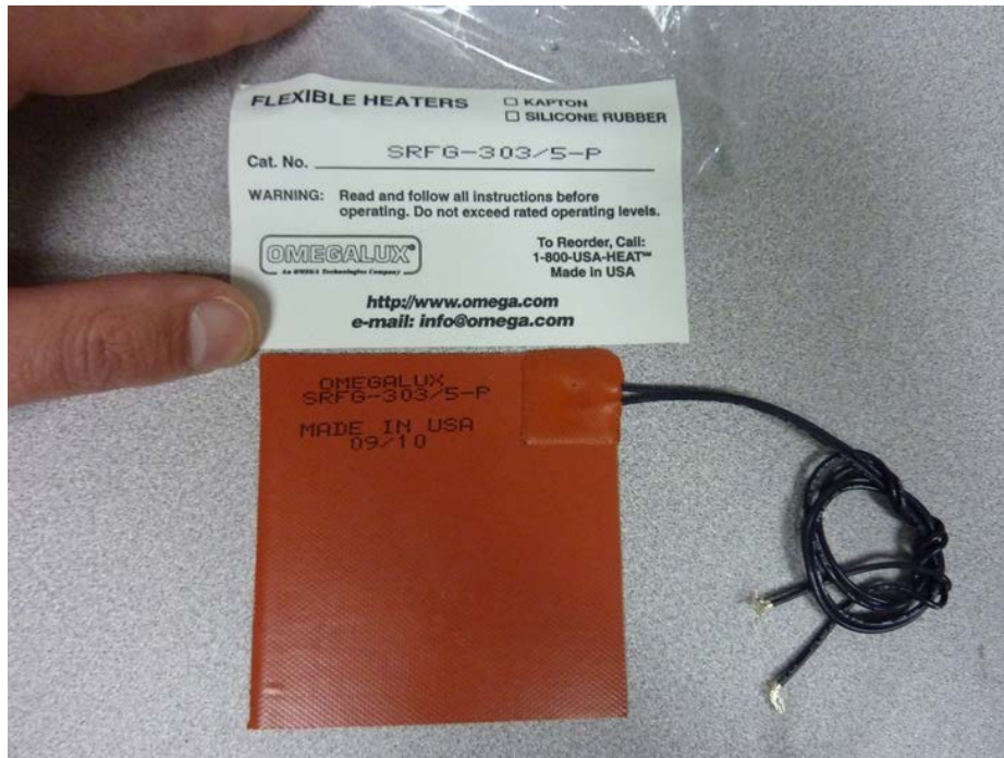
Adhesive Heater
