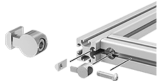
Anchor (Drill an installation hole in the face of one rail to install.)
