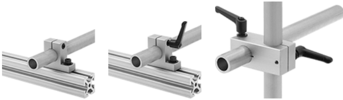
Rail-to-Tube Adjustable Rail-to-Tube Adjustable Tube-to-Tube
