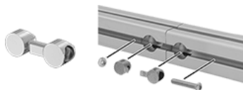
Double Anchor (Drill an installation hole in the face of each rail to install.)
