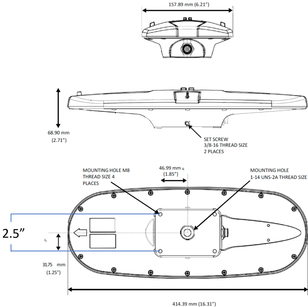
Figure 2-6: V102 dimensions
