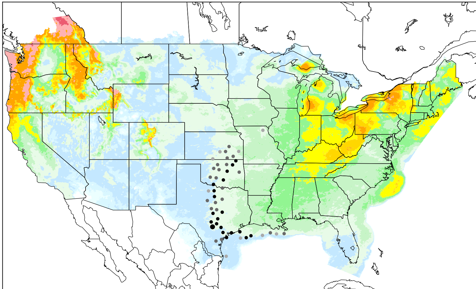
Feb NDFD supp. locations and fraction of climatology with nonzero precipitation
