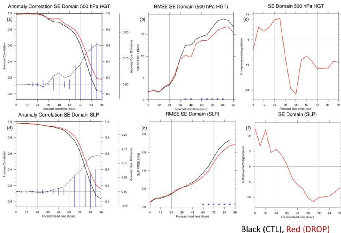
Figure 2.21. Impact of assimilation of Global Hawk dropsondes (DROD) versus the control (CTL) model on anomaly correlation scores and root mean squared error (RMSE) from GFS forecasts during Hurricane Matthew relative to the full observing system. The left panels show the anomaly correlation, the center panels display the RMSE, and the right panel shows the percent change in the RMSE as a function of forecast lead time. Upper panels are for the 500 hPa height field (HGT) and lower panels are for the sea level pressure (SLP). The results reflect averages from three model cycles and over the southeast (SE) verification region. In the anomaly correlation plots, differences (dashed lines) outside of blue vertical lines are significant at the 95% confidence level. Blue stars in the RMSE plots indicate lead times that are statistically significant at the 95% level. Graphics provided by the GOSA Group as appearing in Kren et al. 2017.
