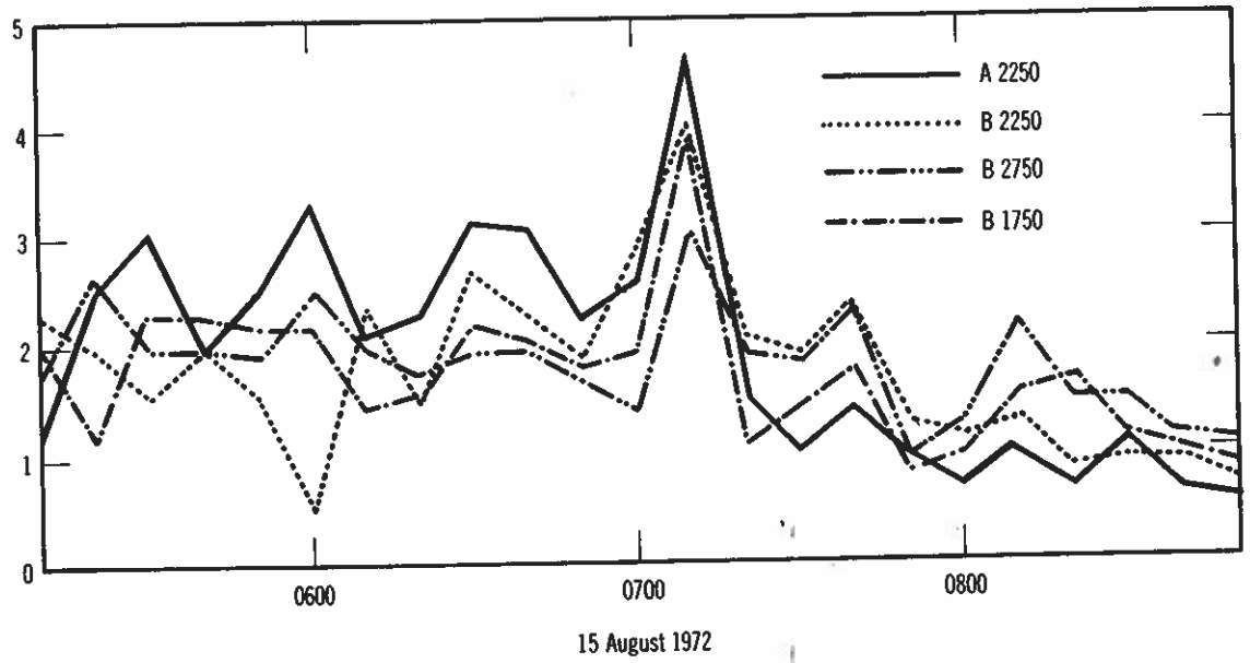
Figure 13. Ratios of echosonde median C_T^2 to tower median C_T^2 for 10-min data blocks for each data channel from 0510 to 0850, 15 August 1972.
