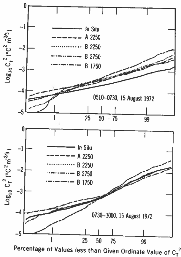
Figure 5. Cumulative probability distributions of C_T^2 obtained from each echosonde and the tower at 92 m. Unfiltered 4-s samples were used in the distributions on 15 August 1972: (a) 0510 to 0730; and (b) 0730 to 1000.
