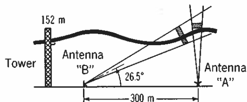
Figure 26. Examination of "turbulent" patches on an isolated layer, utilizing vertical and tilted echosondes from 0636 to 0659, 12 August 1972.
