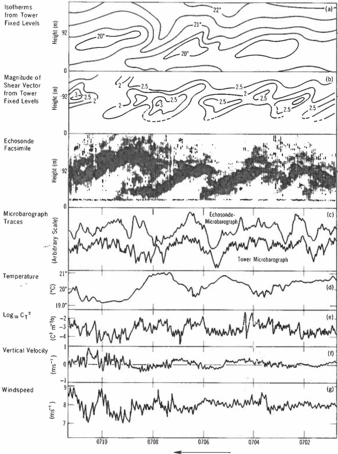
Figure 17. Echosonde facsimile record from 0702 to 0712, 16 August 1972: (a) isotherms obtained from fixed-level temperature data; (b) isopleths of shear vector magnitudes computed from 10-s averages at each fixed level ( = |\vec{v}_i - \vec{v}_{i+1}| ; " \vec{v} " denotes the fixed levels taken at 30.48-m intervals); (c) microbarograph traces obtained at the echosonde and tower with zero time lag; (d) 92-m temperature trace showing a lag relative to the measurement of \frac{\partial p}{\partial t} from the microbarograph; (e) tower C_T^2 trace showing bursts as the instabilities move past the tower; (f) vertical velocity trace (note the 90^\circ phase lag relative to the temperature data); and (g) windspeed.
