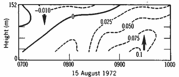
Figure 8. Isopleths of temperature flux Q = \overline{w'T'} ( ^{\circ}\text{C ms}^{-1} ), derived from the fixed-level tower data. Temperature data were detrended using a 20-min running average.
