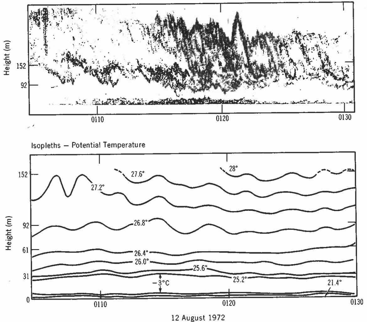
Figure 24. Facsimile detail for period from 0104 to 0132, 12 August 1972, obtained with a pulse repetition period of 2 s and a pulse length of 6 ms and compared with potential temperature contours that were obtained using fixed-level tower data.
