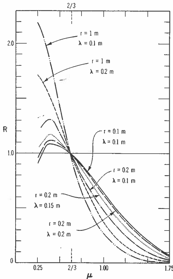
Figure 2. Using the power-law dependence [(\Delta T)^2] \propto r^\mu , we have plotted the ratio R = \sigma(\mu, \lambda) / \sigma(\mu = 2/3, \lambda) as a function of \mu for several values of r and \lambda ( r is the separation of the temperature sensors, \lambda is the acoustic wavelength, and \sigma(\mu, \lambda) is the acoustic scattering cross section per unit volume).
