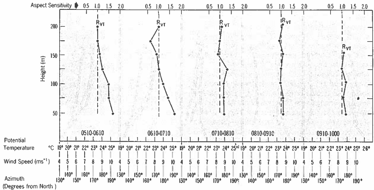
Figure 22. Hourly averaged profiles from the tower fixed levels of windspeed, azimuth, and potential temperature for 15 August 1972 case, with the corresponding ratio R_{VT} , of vertical echosonde C_T^2 to tilted echosonde C_T^2 at 2250 Hz.
