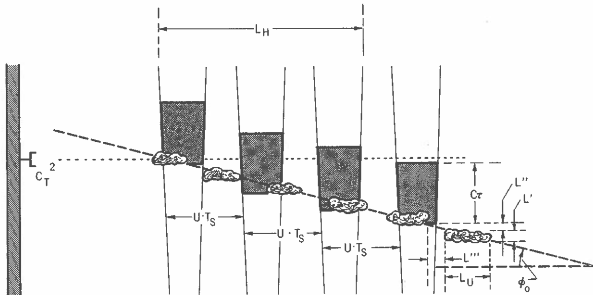
Figure 28. Schematic diagram for computation of the relative echosonde-tower error. The shaded area represents the observed echo within a fixed range gate for a pulse length c\tau .
