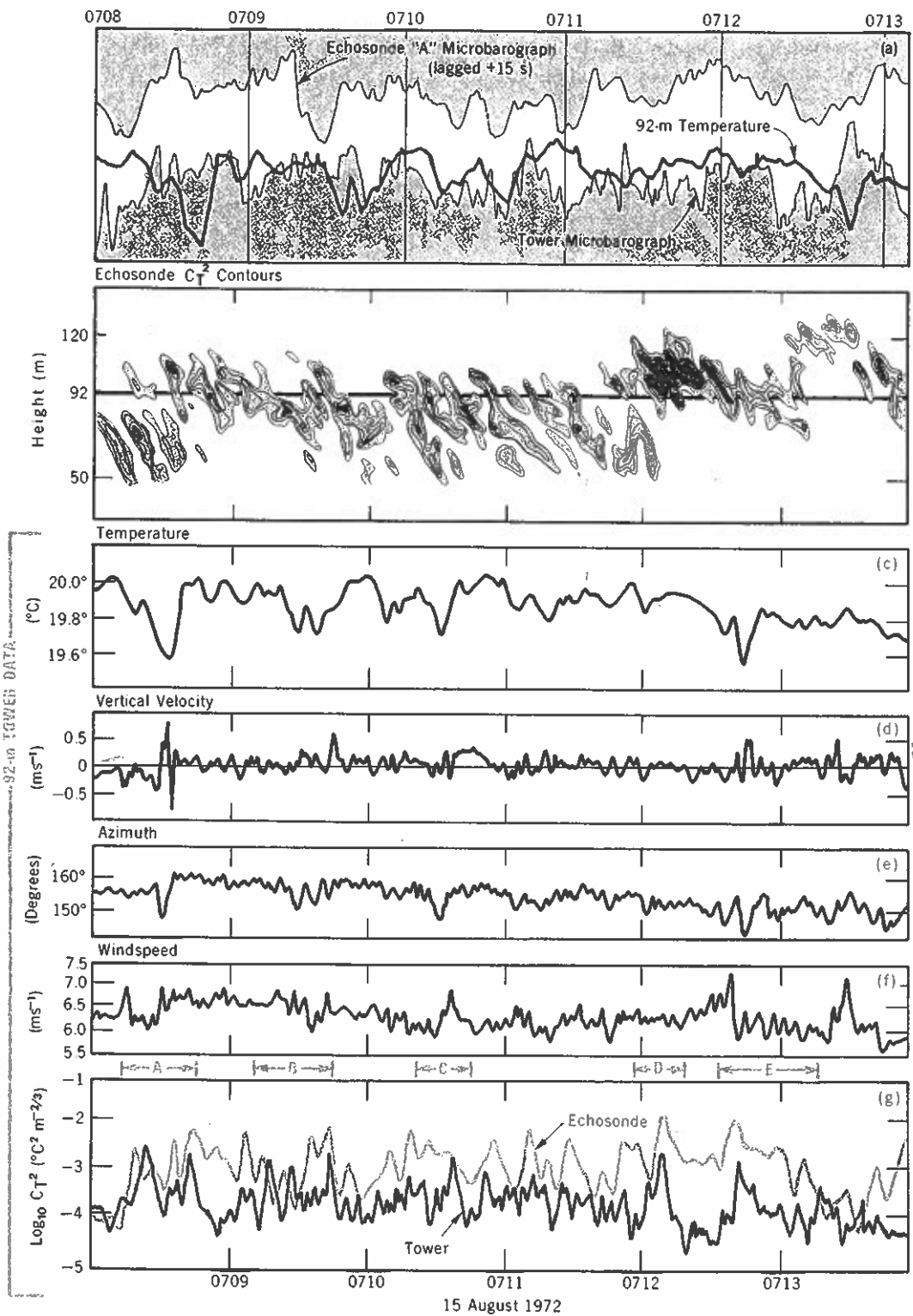
Figure 18. Detailed echosonde contours (3-dB increment in C_T^2 isopleths; minimum equals 0.00125^\circ\text{C m}^{-2/3} ) for period from 0708 to 0713, 15 August 1972: (a) microbarograph at tower base compared with pressure recording at echosonde "A" lagged 15 s; and compared with temperature variation at 92-m level (microbarograph output is proportional to p(t) and \frac{\partial p(t)}{\partial t} , depending on the period of the motion); (c) 92-m tower time series of temperature; (d) 92-m tower time series of vertical velocity; (e) 92-m tower time series of azimuth from north; (f) 92-m tower time series of windspeed; and (g) 92-m tower time series of in situ C_T^2 .
