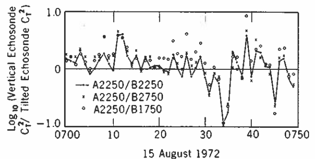
Figure 19. Examination of the aspect sensitivity of the scattering, using ratios of vertical echosonde C_T^2 to tilted echosonde C_T^2 , taken from 1-min averages in the period from 0700 to 0750, 15 August 1972, at 92 m.
