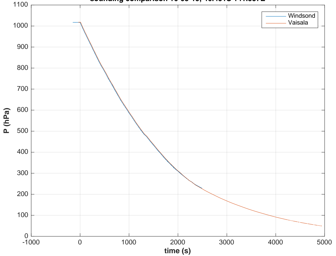
sounding comparison 16-03-19, 46.491S 141.557E
