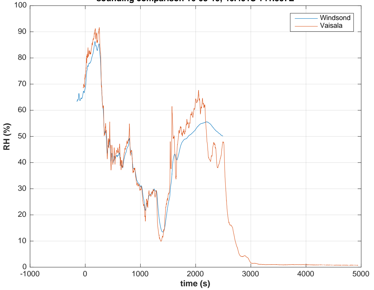
sounding comparison 16-03-19, 46.491S 141.557E
