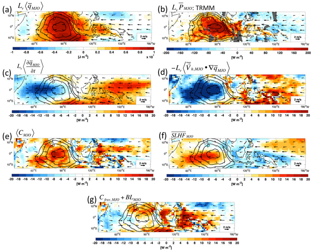
FIG. 2. Composite anomalies of (a) column specific humidity, (b) TRMM precipitation, (c) moisture tendency, (d) horizontal moisture advection, (e) column process, (f) SLHF, and (g) the sum of C_{\text{free}} and BL . Terms (a)–(e), (g) have been multiplied by the latent heat of vaporization. Solid (dashed) contours correspond to positive (negative) NOAA OLR anomalies every 5 \text{ W m}^{-2} beginning at \pm 15 \text{ W m}^{-2} . Arrows indicate ERA-Interim 850-hPa horizontal wind anomalies, and a reference arrow is provided in the lower-right corner. Please note that composites (a) and (c)–(h) result from 75 independent events for 1980–2011, while composite (b) results from 28 events for 1999–2011, and that the color bar in (b) spans from -200 to 200 \text{ W m}^{-2} . Stippling in (b) indicates missing TRMM data. The subscript MJO indicates bandpass filtering to 20–100 days. See text for description of compositing technique.
