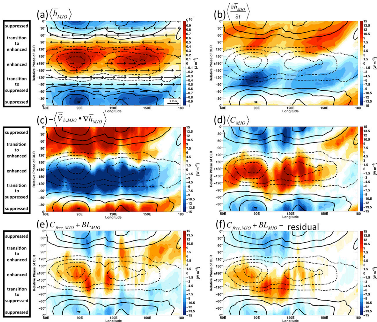
FIG. 11. As in Fig. 3, but color shading for anomalies of (a) column MSE, (b) column MSE tendency, (c) column horizontal advection of MSE, (d) column process, (e) the sum of C_{\text{free}} and BL , and (f) the sum of C_{\text{free}} and BL minus the MSE budget residual. The subscript MJO indicates bandpass filtering to 20–100 days.
