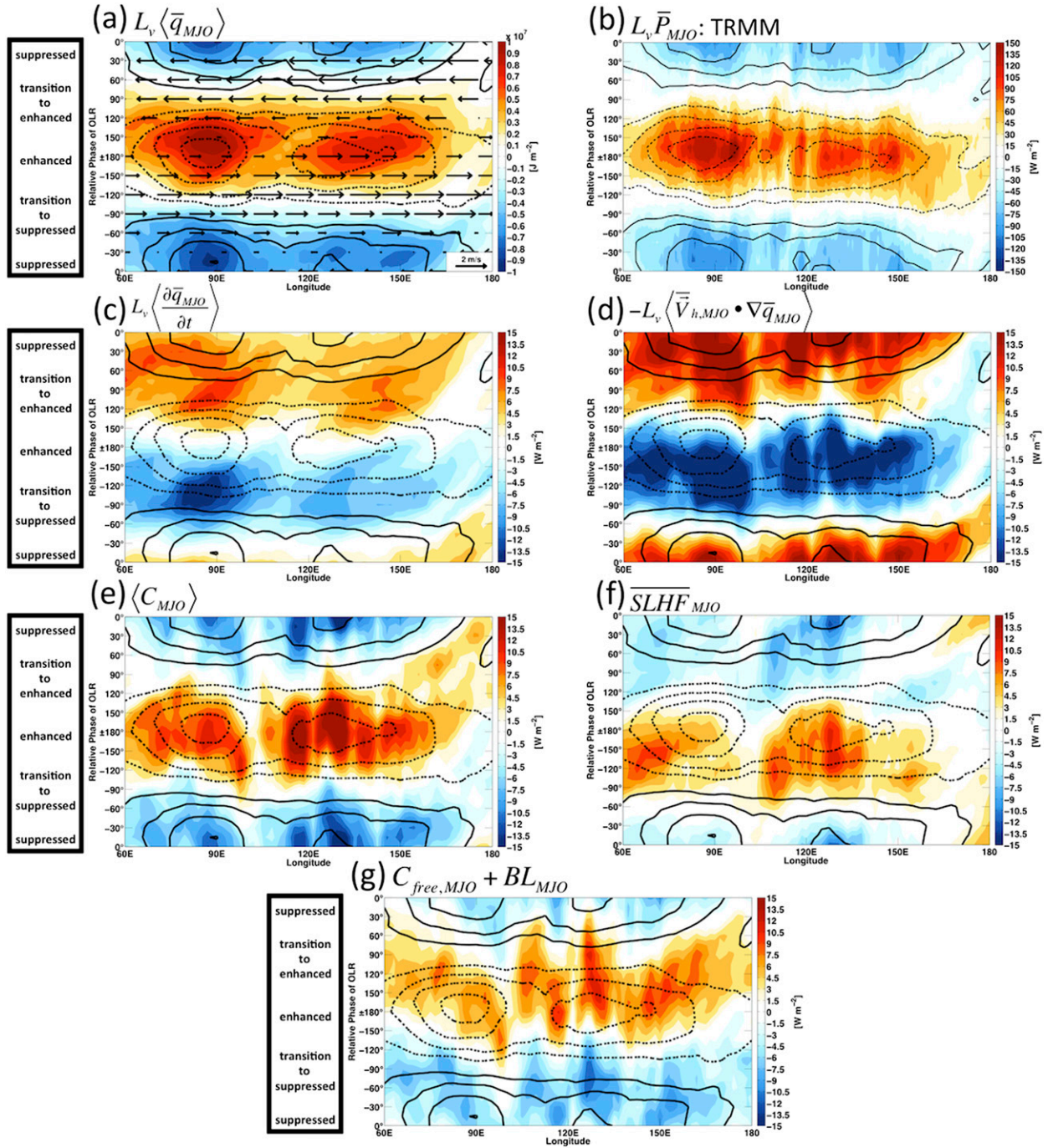
FIG. 3. Composite of (a) latitudinally averaged ( 13.5^{\circ}\text{N} – 13.5^{\circ}\text{S} ) ERA-Interim column latent heat, (b) TRMM precipitation, (c) column latent heat tendency, (d) column horizontal advection of latent heat, (e) column process, (f) SLHF, and (g) the sum of C_{\text{free}} and BL as a function of relative phase of OLR. Solid (dashed) contours correspond to positive (negative) NOAA OLR anomalies every 6 \text{ W m}^{-2} beginning at \pm 6 \text{ W m}^{-2} . Arrows in (a) indicate ERA-Interim U850 anomalies, and a reference arrow is provided in the lower-right corner. Moving downward from the top of the figure corresponds with the transition from suppressed convection (top of the figure, positive OLR anomalies) to enhanced convection (middle of the figure, negative OLR anomalies), and back to suppressed convection (bottom of the figure, positive OLR anomalies) at each longitude. The subscript MJO indicates bandpass filtering to 20–100 days. See text for description of compositing technique.
