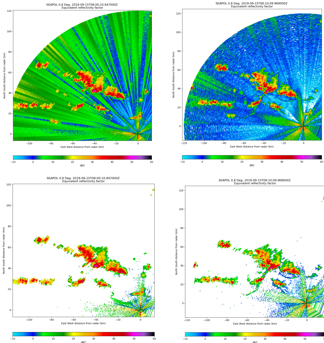
Fig. E1: Example of echoes with HiSeas Net antenna “active” (left) and “pointed away” (right). Echoes are 10 minutes apart at 0.8 deg elevation. Bottom: Same as above, but filtered using NCP \geq 0.45 and \rho_{hv} > 0.7 .
