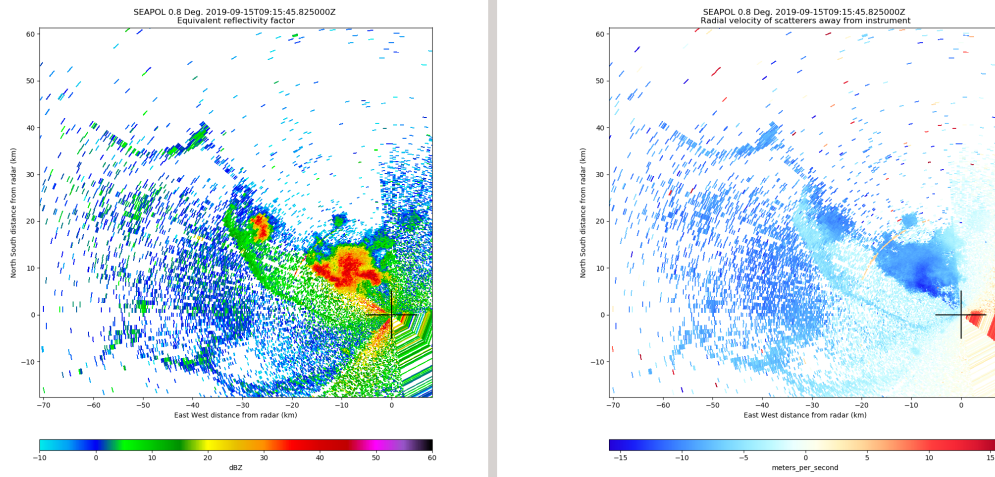
Fig. 6: Boundaries on the low-level surveillance scan at 0915 UTC.
