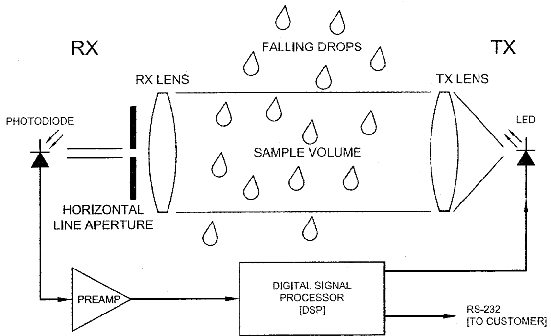
Figure 3.1 ORG 815 Sensor Block Diagram
