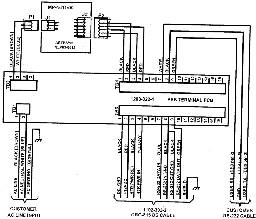
Figure 2.4 Power Supply Box Wiring Connections for ORG 815 DS Series
