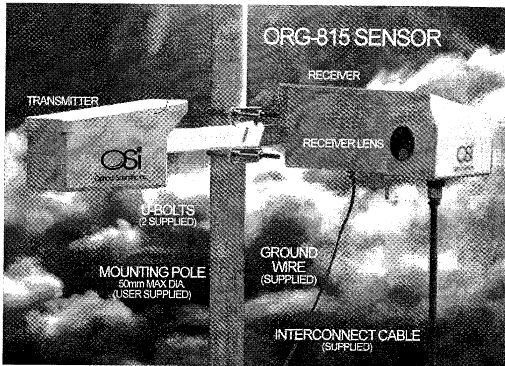
Figure 1.3 ORG-815-DS Major Components
