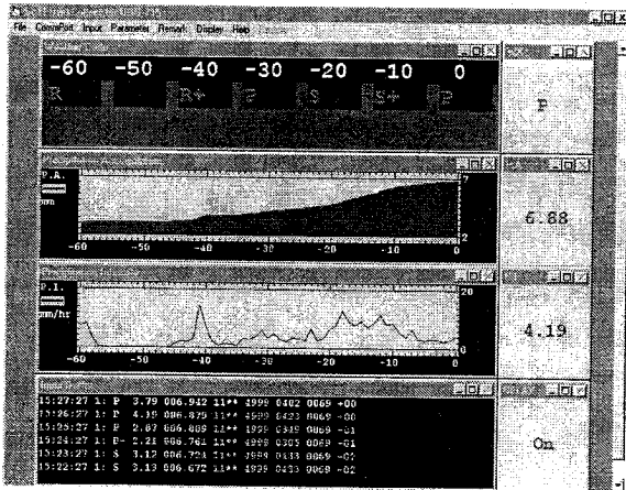
Figure 1.5 QwikCollect Software
