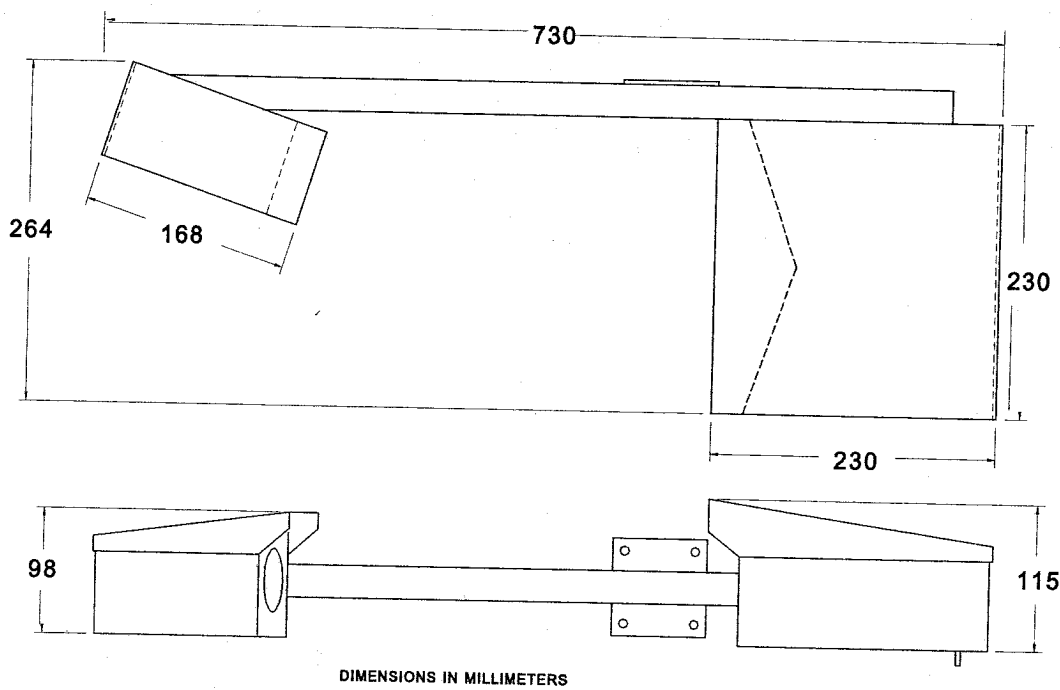
Figure 1.2 ORG-815-DS Dimensions
