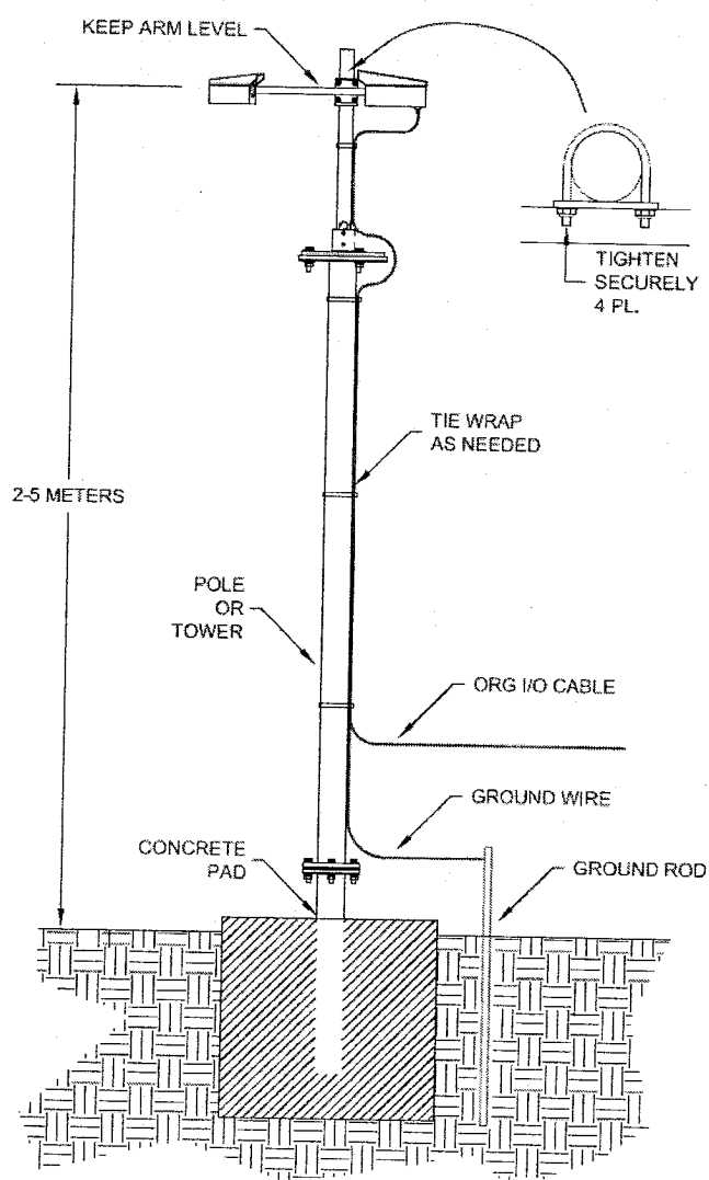
Figure 2.2 Typical ORG Installation
