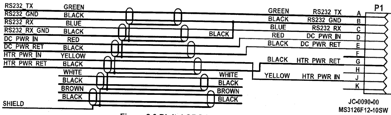
Figure 2.3 Digital ORG Interconnect Cable
