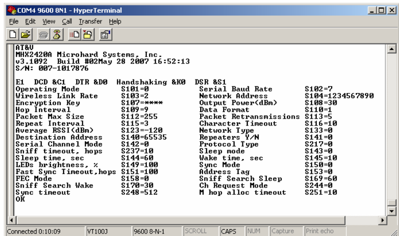
Image 5: &F1 PMP Master Configuration View
