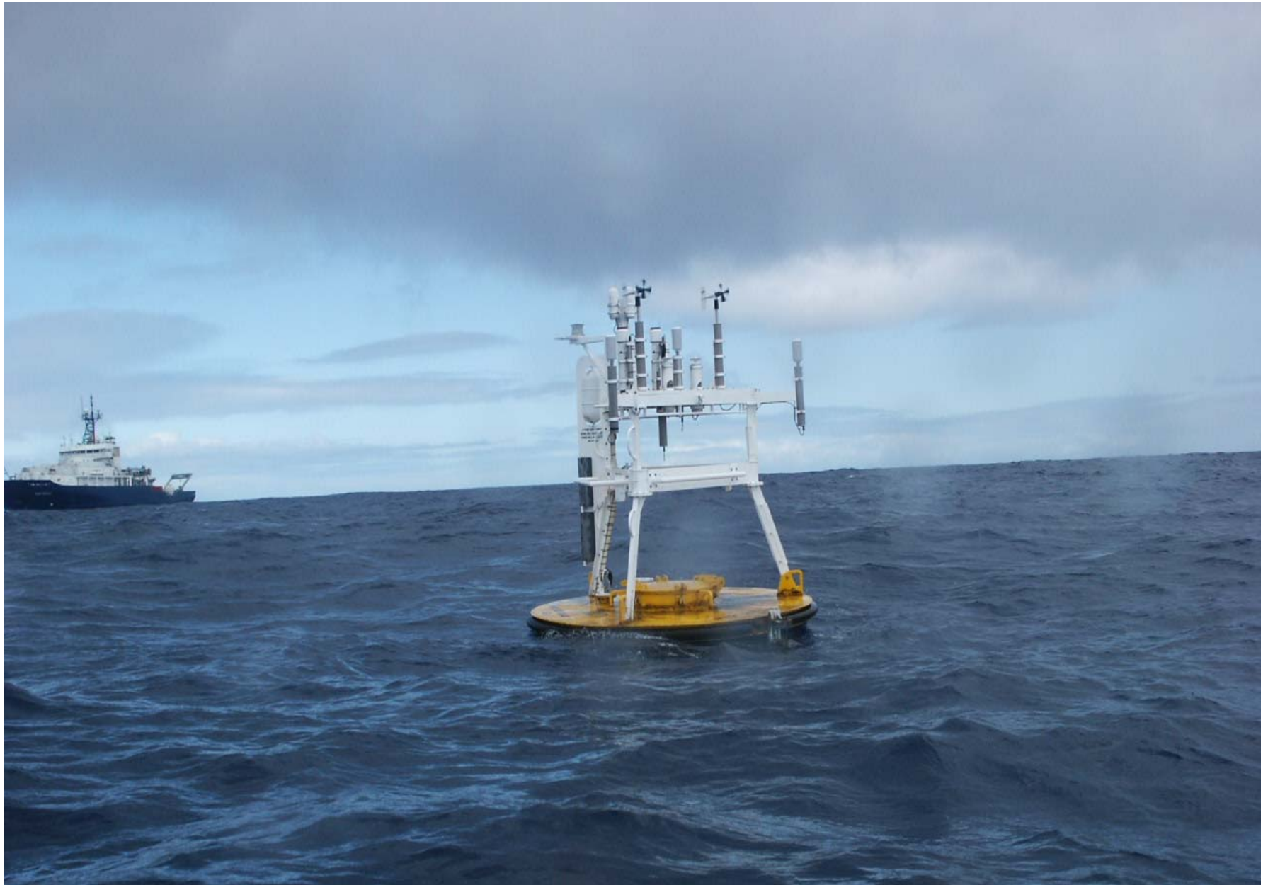
Figure 2. The old WHOI buoy awaiting replacement after a year on the job.
