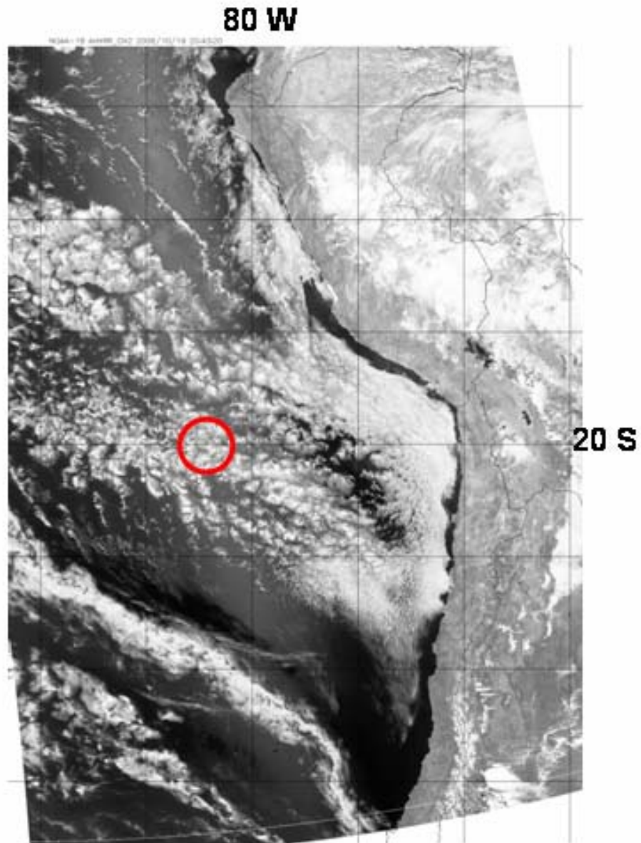
Figure 31. Terascan satellite visible image NOAA-18 2043 UTC October 19, 2006. Red circle is the location of the STRATUS buoy (20 S, 85W)
