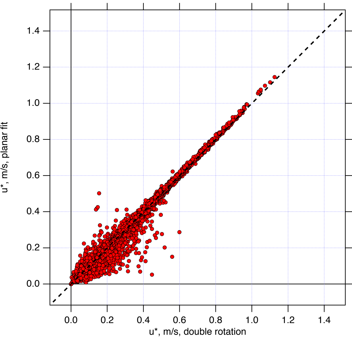
Friction Velocity Comparison, 3m
